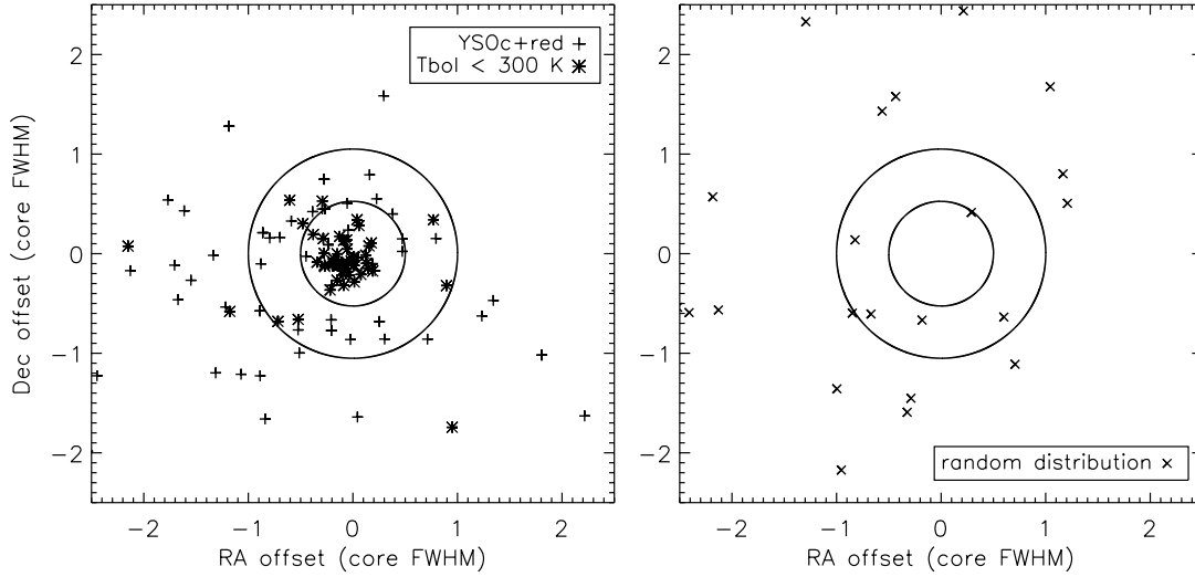
FIG. 2.— Left : Distribution of the positional offset from each protostar candidate in Perseus to the nearest 1.1 mm core centroid. Distances are in units of the core FWHM size ( \theta_{1\text{ mm}} ), and circles enclose sources within 0.5 and 1.0 \times \theta_{1\text{ mm}} of a core position. Pointing errors in the Bolocam maps are typically 10'' or less. Protostar candidates include all “YSOc,” “red,” and 70\ \mu\text{m} sources, while candidates with bolometric temperatures T_{\text{bol}} < 300\ \text{K} (M. L. Enoch et al. 2008, in preparation) are shown in bold. These cold objects, which are most likely to be most embedded, are primarily located within 1.0 \times \theta_{1\text{ mm}} of a core centroid. Right : Expected distribution if the IR sources were distributed randomly over the Bolocam map area (i.e., if they were not spatially correlated with the cores). Our definition that a given 1.1 mm core is protostellar if there is a candidate protostar within 1.0 \times \theta_{1\text{ mm}} of the core position will result in a few false associations in each cloud.
