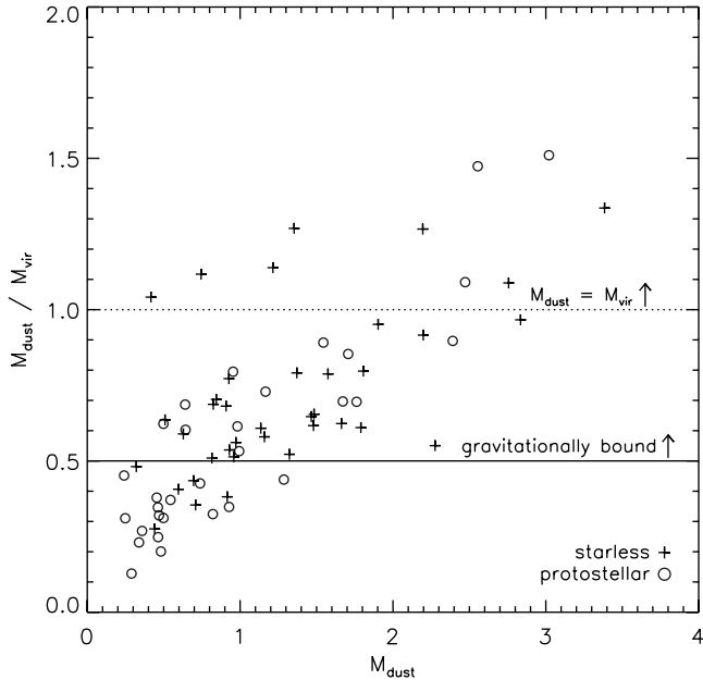
FIG. 12.—Ratio of the total mass derived from dust ( M_{\text{dust}} ) to the virial mass ( M_{\text{vir}} ), calculated using the temperature and velocity dispersion derived from GBT \text{NH}_3 (1, 1) and (2, 2) observations (Rosolowsky et al. 2008), for starless and protostellar cores in Perseus. Only those with well-determined \text{NH}_3 line widths are shown. Lines indicate the minimum M_{\text{dust}}/M_{\text{vir}} for which cores should be in virial equilibrium (dashed line) or self-gravitating (solid line). [See the electronic edition of the Journal for a color version of this figure.]
