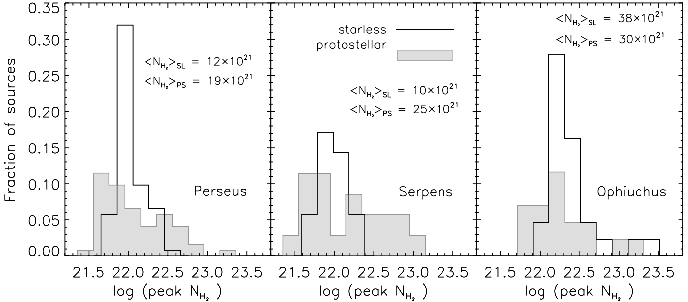
FIG. 6.—Distributions of the peak column density N_{\text{H}_2} of starless and protostellar cores. The peak N_{\text{H}_2} values of starless cores are considerably lower than those of protostellar cores in both Perseus and Serpens, by factors of approximately 1.6 and 2.5, respectively. In Ophiuchus there is no significant difference in the mean values, but in all three clouds the starless distribution is confined to a narrowly peaked distribution.
