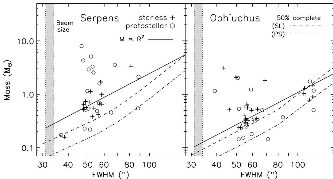
FIG. 9.—Total mass vs. angular FWHM size for starless and protostellar cores in Serpens and Ophiuchus. Lines are as in Fig. 8; as for Perseus, the 90% completeness curves are approximately a factor of 1.2 higher in mass than the 50% completeness curves, although they are omitted here for clarity. Unlike in Perseus, starless cores do not necessarily follow a constant-surface-density ( M \propto R^2 ) line. Strikingly, there is no population of large starless cores in Serpens; it is not clear how the current population of relatively massive protostellar cores could have evolved from such compact, low-mass starless cores. This discrepancy suggests that future star formation in the cloud may result in stars of considerably lower mass than the currently forming protostars. [See the electronic edition of the Journal for a color version of this figure.]
