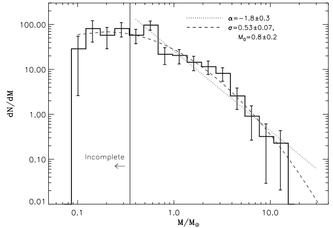
FIG. 15.—Combined protostellar mass distribution, with power-law and log-normal fits. The protostellar CMD includes all protostellar cores from Perseus, Serpens, and Ophiuchus, and the 50% mass completeness limit is defined by the completeness to average-sized protostellar cores in Perseus. The best-fit power law ( \alpha = -1.8 ) is shallower, and the distribution as a whole is wider, than the prestellar CMD (Fig. 13). This difference is expected if the protostellar CMD evolved from the prestellar CMD. The fact that the protostellar distribution extends to higher masses than the prestellar CMD is more difficult to explain, however, and may suggest that higher mass prestellar cores are relatively short lived. [See the electronic edition of the Journal for a color version of this figure.]
