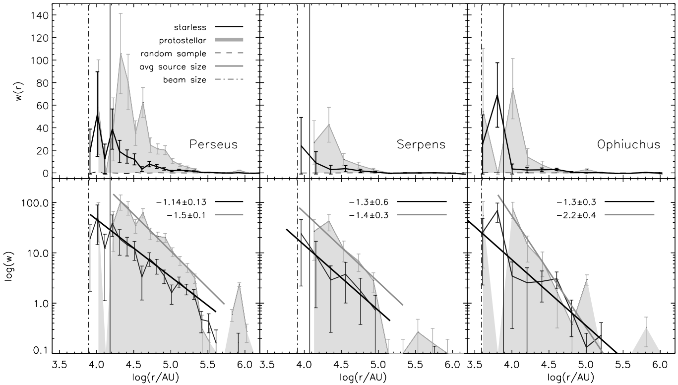
FIG. 11.—Two-point spatial correlation function w(r) , plotted as a function of source separation r , for starless and protostellar cores in Perseus, Serpens, and Ophiuchus ( top panels ). Bottom panels plot \log(w) , with the best-fitting power-law slope for each distribution. Resolution limits and average source sizes are indicated. Power-law slopes are fit for r larger than the average source size in each cloud. The amplitude of the protostellar w(r) is consistently higher than the starless w(r) , indicating that clustering of protostellar cores is stronger on all spatial scales. Slopes for the starless and protostellar populations are similar in each cloud, however, so although the magnitude of clustering differs, the fundamental nature of the clustering does not.
