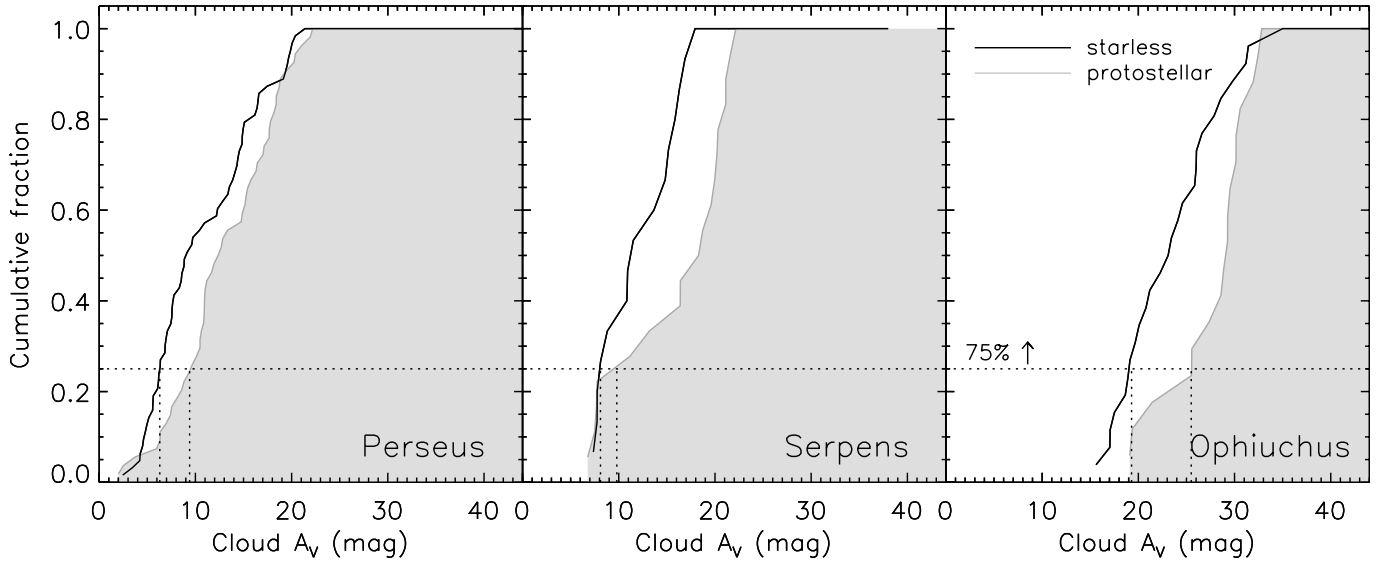
FIG. 10.—Cumulative fraction of starless and protostellar cores as a function of cloud A_V , where the A_V is derived from the reddening of background stars in 2MASS and IRAC data. In all three clouds, the majority of cores are found at high cloud column densities ( A_V > 7 mag). Dotted lines indicate the A_V at which >75\% of cores are found; 75\% of starless and protostellar cores in Perseus are located at A_V \gtrsim 6.5 and 9.5 mag, respectively. The equivalent values are A_V \gtrsim 6 and 10 mag in Serpens, and A_V \gtrsim 19.5 and 25.5 mag in Ophiuchus. There appears to be a strict extinction threshold in Serpens and Ophiuchus, with no cores found below A_V \sim 7 and 15 mag, respectively.
