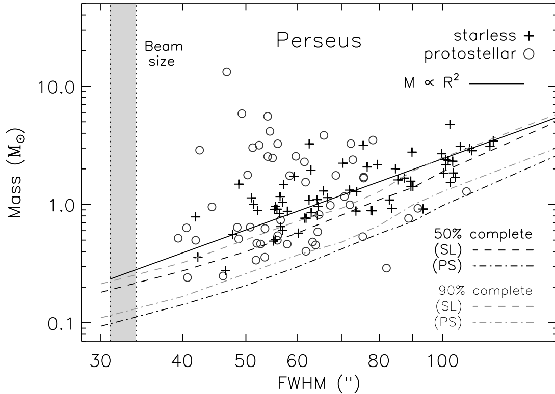
FIG. 8.—Total mass vs. angular FWHM size for starless and protostellar cores in Perseus. Dashed and dash-dotted lines indicate empirically derived 50% (and 90%; light gray ) completeness limits for starless and protostellar cores, respectively. The two populations seem to inhabit different regions of the parameter space: starless cores tend to follow a constant-surface-density relationship ( M \propto R^2 ; solid line ), consistent with their narrow distribution in column density (Fig. 6), while protostellar cores have a wide range in masses for a relatively small range in sizes. This relationship suggests a simple explanation for how the protostellar cores might have evolved from a similar population of starless cores, with individual cores becoming smaller and denser at a constant mass until protostar formation is triggered. [See the electronic edition of the Journal for a color version of this figure.]
