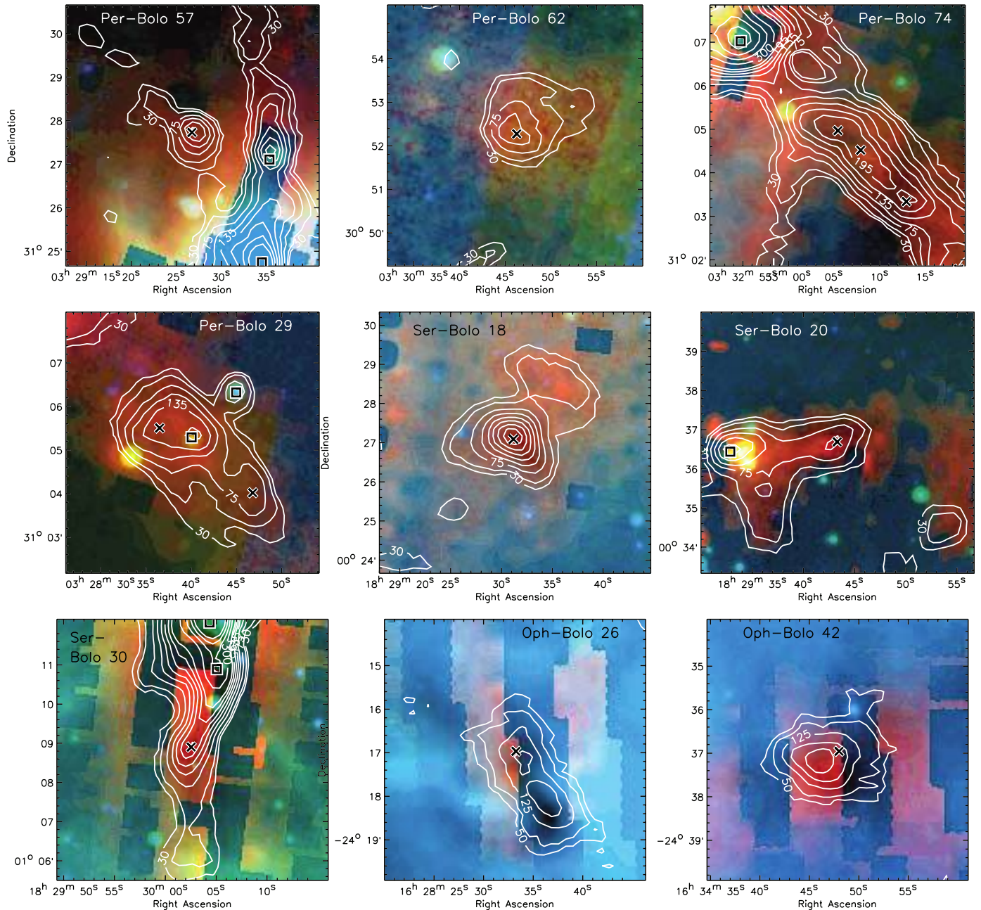
FIG. 1.— Three-color Spitzer images (8.0, 24, 160 \mu\text{m} ) of selected starless and protostellar cores in Perseus, Serpens, and Ophiuchus. Bolocam 1.1 mm contours are overlaid at intervals of 2, 3, 5, . . . , 35 \sigma , where 1 \sigma is the mean rms noise in each 1.1 mm Bolocam map (15 mJy in Perseus, 10 mJy in Serpens, and 25 mJy in Ophiuchus). Positions of starless cores are indicated by an cross, protostellar cores by a square, and the Bolocam ID of the centered core is given. Note the lack of infrared point sources near the starless core positions. Starless cores are most notable in the infrared by their extended 160 \mu\text{m} emission or dark shadows at shorter wavelengths, while protostellar cores are clearly associated with Spitzer point sources. Saturation, image artifacts, and incomplete sampling causes the striped appearance of some of the red 160 \mu\text{m} images.
