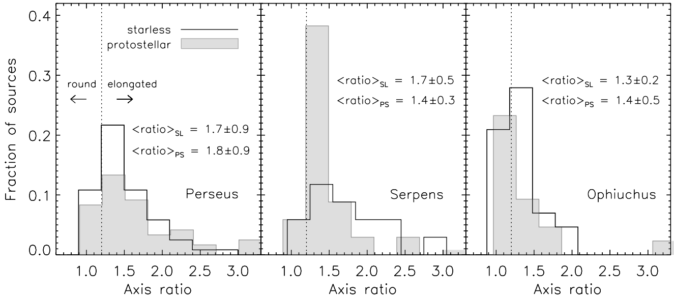
FIG. 5.—Distributions of the axis ratios of starless and protostellar cores. Cores with axis ratios <1.2 are considered round and those with axis ratios >1.2 elongated, based on Monte Carlo simulations (Paper I). Only in Serpens, where starless cores tend to be slightly more elongated than protostellar cores, is there a distinguishable difference between the starless and protostellar populations.
