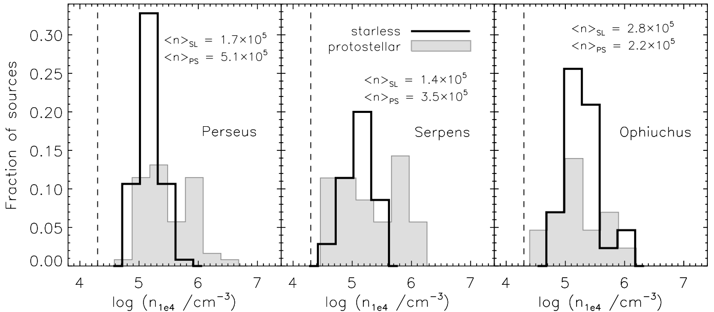
FIG. 7.—Distributions of the mean density n_{1e4} of starless and protostellar cores, where the density is calculated in a fixed linear aperture of diameter 10^4 AU (§ 3.2). As for the peak N_{H_2} distribution (Fig. 6), starless cores tend to have lower mean densities than protostellar cores in Perseus and Serpens, by approximately a factor of 3. In Ophiuchus, by contrast, there is almost no difference between the two distributions. Note that the Bolocam surveys are only sensitive to relatively dense cores with n \gtrsim 2 \times 10^4 \text{ cm}^{-3} (dashed lines; see Paper III).
