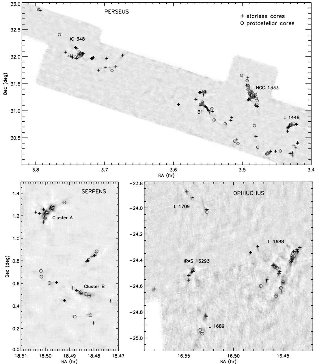
FIG. 3.—Bolocam maps of Perseus, Serpens, and Ophiuchus, with the positions of starless and protostellar cores indicated. Identified cores have peak flux densities of at least 5\sigma , where \sigma is the local rms noise level (on average \sigma = 15 \text{ mJy beam}^{-1} in Perseus, 10 \text{ mJy beam}^{-1} in Serpens, and 25 \text{ mJy beam}^{-1} in Ophiuchus). Note that due to the large scales, individual structures are difficult to see. Regions of the maps with no detected sources have been trimmed for this figure. Starless and protostellar cores cluster together throughout each cloud, with both populations tending to congregate along filamentary cloud structures. There are a few exceptional regions, however, which are dominated by either starless or protostellar cores (e.g., the B1 ridge, Serpens cluster A). [See the electronic edition of the Journal for a color version of this figure.]
