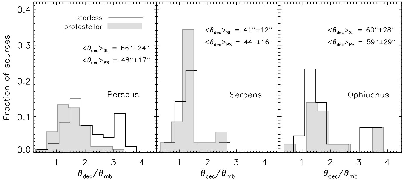
FIG. 4.—Distributions of the angular deconvolved sizes of starless and protostellar cores in the three clouds. The size is given in units of the beam FWHM ( \theta_{\text{mb}} ), and the mean of each distribution \pm the dispersion in the sample is listed. Starless cores are larger on average than protostellar cores in Perseus, with a flattened distribution out to 3.5\theta_{\text{mb}} . In Serpens and Ophiuchus, however, there is little difference between the starless and protostellar distributions, and there are fewer very large cores, particularly in Serpens. The value of \theta_{\text{dec}}/\theta_{\text{mb}} can be used to infer the steepness of the source radial density profile (see text and Young et al. 2003).
