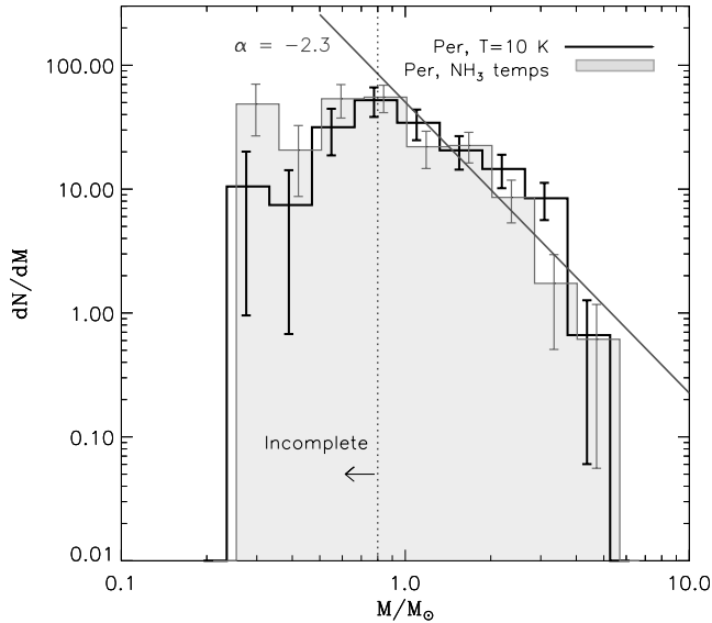
FIG. 14.—Effect on the prestellar CMD in Perseus of using \text{NH}_3 -derived core kinetic temperatures (shaded histogram) rather than assuming a constant T_D = 10 K for all cores (black histogram). Only starless cores in Perseus are included here. The best-fitting power-law slope for M > 0.8 M_\odot is similar for the two histograms: \alpha = -2.35 \pm 0.33 and \alpha = -2.33 \pm 0.28 for the T_D = 10 K and \text{NH}_3 temperature curves, respectively. Although we do not have kinetic temperatures for cores in Serpens or Ophiuchus, we do not expect temperature effects to dramatically alter the derived prestellar CMD slope.
