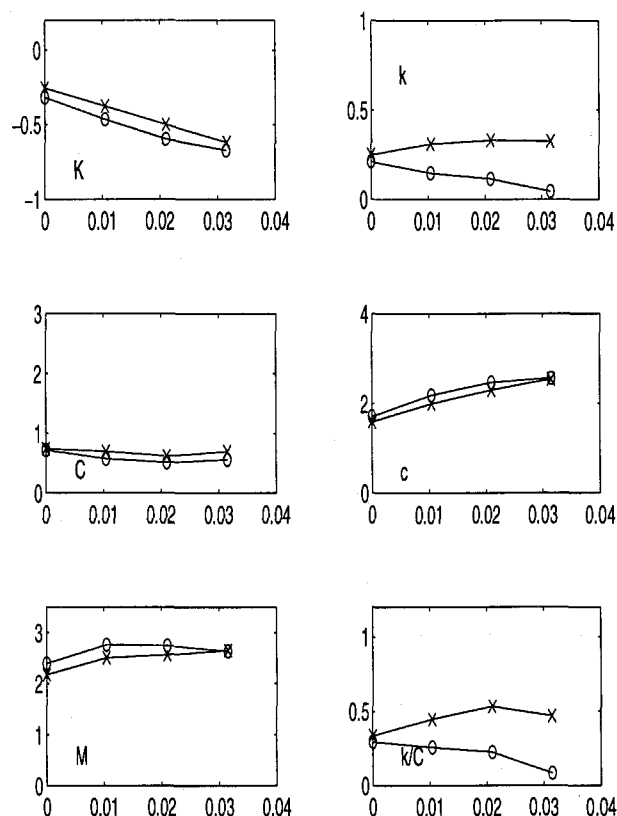
FIGURE 4: Rotordynamic force coefficients as functions of the flow coefficient \phi for experimental tests with the conical (o) and contoured shroud (x).
