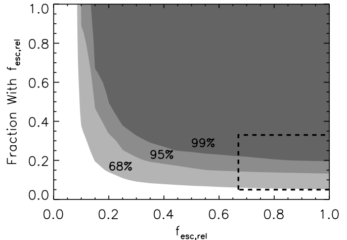
FIG. 11.—Parameter space excluded by a Monte Carlo analysis of the combined limits of this work with M03. The x-axis is the relative escape fraction, and the y-axis is the fraction of galaxies that have this escape fraction. The other galaxies are assumed to have negligible escape fractions. The shaded regions are excluded (at 3, 2, and 1 \sigma ; darker to lighter) by the fact that we detect no galaxies in the combined sample of 32 galaxies. The dashed box denotes the approximate parameter space implied by S06. The horizontal errors to the box are from uncertainties in the determination of the relative escape fraction, and the vertical errors are Poisson.
