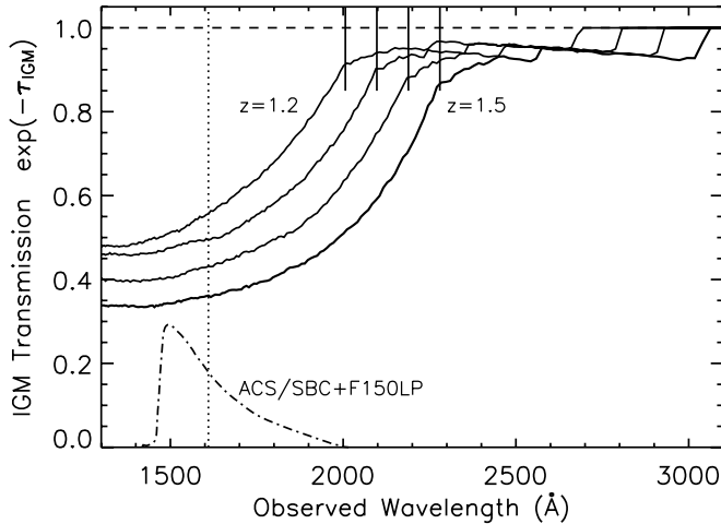
FIG. 2.—Average transmission through the IGM of UV light from galaxies at redshift 1.2, 1.3, 1.4, and 1.5 (left to right). Each curve is computed from simulations along 1000 LOSs through the Ly \alpha forest. The corresponding Lyman limits are denoted by solid vertical lines. As a reference, the transmission curve is plotted for the ACS SBC F150LP filter used in our observations (dot-dashed line). The vertical dotted line is the pivot wavelength of the filter curve.
