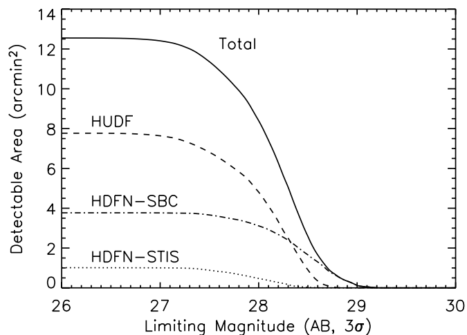
FIG. 6.—Detectable area as a function of limiting magnitude (AB, 3\sigma ) within a 1'' diameter circular aperture. The solid line is the total area from all three surveys. The dashed, dotted, and dot-dashed lines are the areas of the HUDF, HDFN-STIS, and HDFN-SBC surveys, respectively. The HUDF survey is much larger, allowing us to detect more objects, while the HDF-SBC survey is deeper. We are sensitive to fainter galaxies if their extraction isophotes are smaller.
