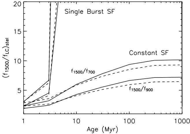
FIG. 1.—The f_{1500}/f_{700} and f_{1500}/f_{900} intrinsic flux ratios as a function of time since onset of star formation using the BC03 (solid lines) and Starburst99 (dashed lines) models.
