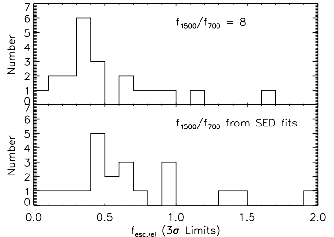
FIG. 8.—Histogram of the f_{\text{esc,rel}} limits of our sample. The top panel limits are derived assuming a UV-to-LC ratio (f_{1500}/f_{700})_{\text{stel}} = 8 , whereas the bottom panel shows the limits derived when taking the UV-to-LC ratio from the best-fit model. Limits of f_{\text{esc,rel}} < 1.0 indicate additional attenuation (by either dust or H I) in addition to the attenuation at 1500 \text{ \AA} . Eighteen (of 21) galaxies have limits of f_{\text{esc,rel}} \leq 1.0 , and nine have f_{\text{esc,rel}} < 0.5 (when using SED fits).
