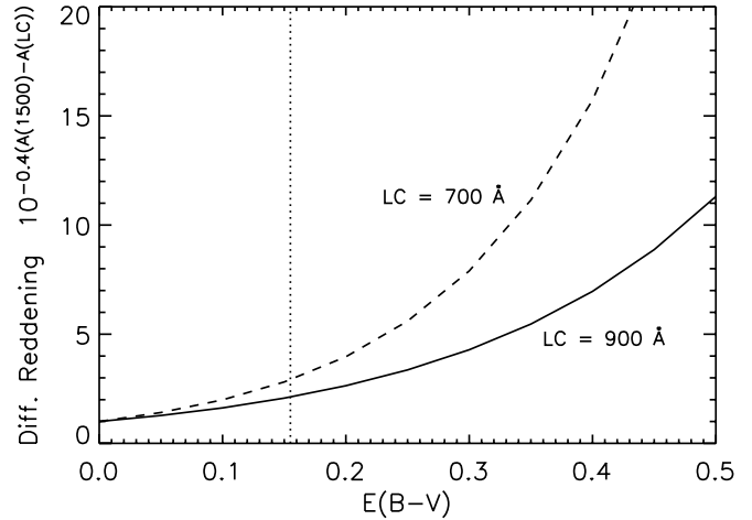
FIG. 4.—Differential reddening from 1500 \text{\AA} and the Lyman continuum (defined as 10^{-0.4[A(1500)-A(LC)]} , where LC is either 900 or 700 \text{\AA} ) as a function of dust reddening for a Calzetti reddening law extrapolated to \lambda = 700 \text{ \AA} . The dotted vertical line shows the median value of E(B - V) = 0.155 for Shapley et al. (2001) for LBGs derived from broadband photometry. The tail of the reddening distribution for LBGs extends out to E(B - V) = 0.4 . The 700 \text{\AA} flux is affected far more than at 900 \text{\AA} , showing that our measurements are more sensitive to dust than those measurements just blueward of the Lyman limit.
