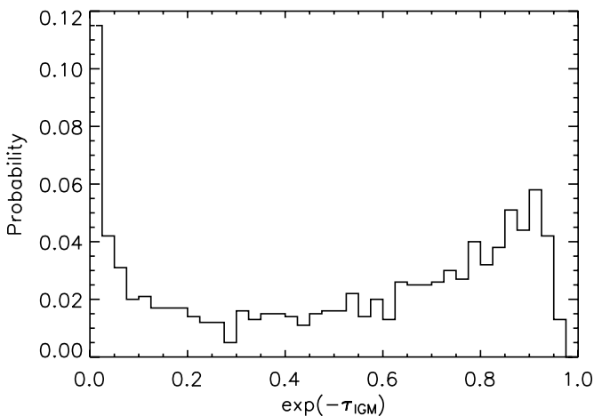
FIG. 3.—Distribution of IGM transmission within the F150LP filter for 1000 LOSs toward galaxies at z = 1.3 . The spike at zero transmission is due to LLSs and DLAs within \Delta z \sim 0.4 from the target galaxy. The mean and median are 0.51 and 0.59, respectively.
