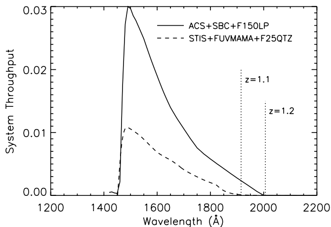
FIG. 5.—Total system throughput for the ACS+SBC+F150LP (solid line) and STIS+FUV-MAMA+F25QZ (dashed line) configurations. The ACS SBC is nearly 3 times more sensitive than the STIS configuration. The dashed vertical lines denote the location of the Lyman limit at z = 1.1 and 1.2 , the low-redshift cutoffs for our sample selection for each configuration.
