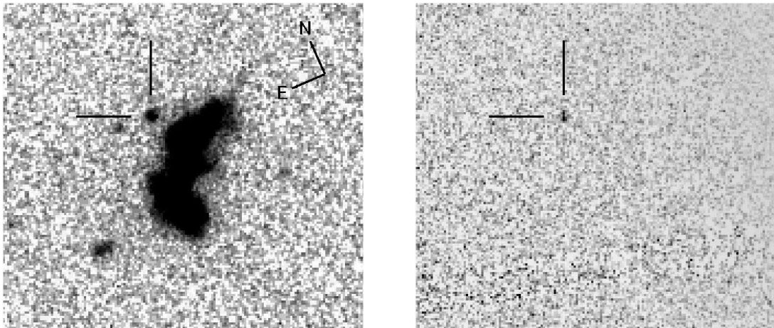
FIG. 10.— HST WFPC2 B -band (F450; left ) and far-UV (F150LP; right ) images of J123652.69+621355.3. The orientation and alignment are the same in both images, and the pointers are in the same location on the sky. The pointers are each 1'' in length and point to the faint source to the north of the target galaxy. The source is clearly detected in the far-UV image.
