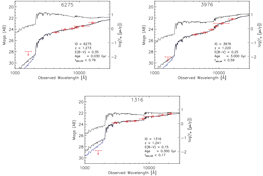
FIG. 9.—Best-fit SEDs for three galaxies. Plotted in each panel are the original SED ( thin line ), with best-fit reddening applied ( thick line ), and with average IGM absorption applied ( blue line ). Top left : This galaxy (J033237.07–274617.3) has no indication of a Balmer break but has a red spectral slope so it is fitted with a young (30 Myr) and dusty [ E(B - V) = 0.35 ] model. Top right : Red galaxy (J033244.16–274729.5) with a prominent Balmer break fitted with a very old (3 Gyr), relatively dusty [ E(B - V) = 0.25 ] template. Bottom : Galaxy (J123643.41+621151.6) with an SED very similar to typical LBGs [age = 300 Myr, E(B - V) = 0.15 ]. The far-UV 3\sigma limits are plotted with downward-pointing arrows. Note that our ability to detect leaking Lyman continuum is largely dependent on the level of dust attenuation.
