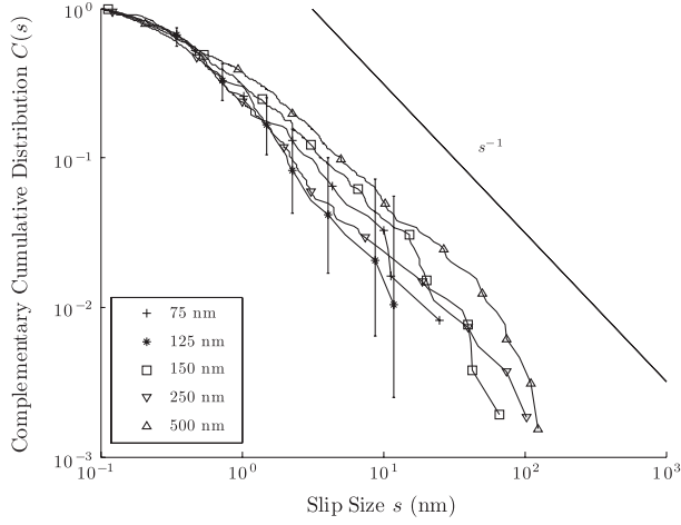
FIG. 4. Stress-integrated cumulative histograms C(S) of the slip size S for various sizes of Cu nanopillars compressed at a displacement rate of 2 nm/s. Larger pillars have larger maximum slip events, except for the 125 nm pillars, for which less data were taken. (For power-law distributions, the largest expected slip size increases with the total number of slips.)
