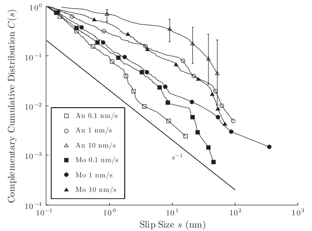
FIG. 3. Stress-integrated cumulative histograms C(S) of slip sizes S for uniaxial compression data: comparison of the impact of nominal displacement rate for Mo and Au pillars of diameter 800 nm. The nominal displacement rate impacts the apparent power laws of the cumulative slip-size histograms. The fitted probability density function exponents are 2.1 \pm 0.1 , 1.45 \pm 0.1 , 1.2 \pm 0.2 , 1.85 \pm 0.1 , 1.8 \pm 0.1 , and 1.6 \pm 0.3 , in the order of the legend (subtract 1 for CDF exponents). The lowest rates are used to compare with model predictions.
