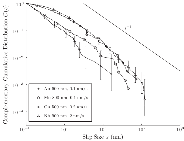
FIG. 2. Stress-integrated cumulative histograms C(S) of slip sizes S (i.e., the fraction of slips with sizes >S plotted versus S ) for uniaxial compression of various materials, pillar sizes, and nominal displacement rates, integrated over stress from zero to critical (failure) stress. C(S) contains hundreds of points (one point per event). Error bars [from Bayesian 95% confidence bounds (see Supplemental Material [14])] are shown for histograms with the most and the least points for clarity. Fitted probability density function power-law exponents: 2.1 \pm 0.1 (Au), 1.85 \pm 0.1 (Mo), 1.8 \pm 0.2 (Cu), and 1.9 \pm 0.2 (Nb) (subtract 1 for CDF exponents). Fits were obtained from maximum likelihood estimates [32] (see Supplemental Material [14] for error bars and fitting techniques for all figures).
