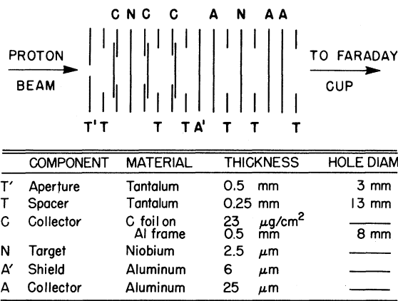
FIG. 1. Schematic diagram of target arrangement used for the sputtering. The entire stack was clamped together, with a total thickness of about 4 mm.
