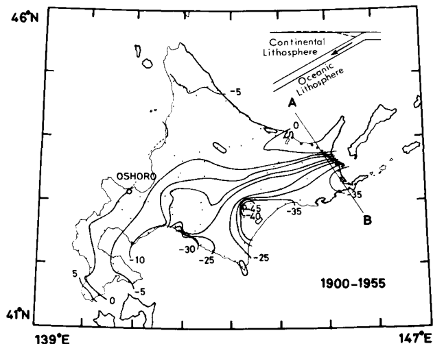
Figure 5. Vertical crustal deformation in Hokkaido, Japan, during the period 1900 to 1955 (unit:cm). Shimazaki's [1974a] model is schematically shown in the inset. Dotted curve shows the deformation due to the drag of the undergoing oceanic lithosphere.
