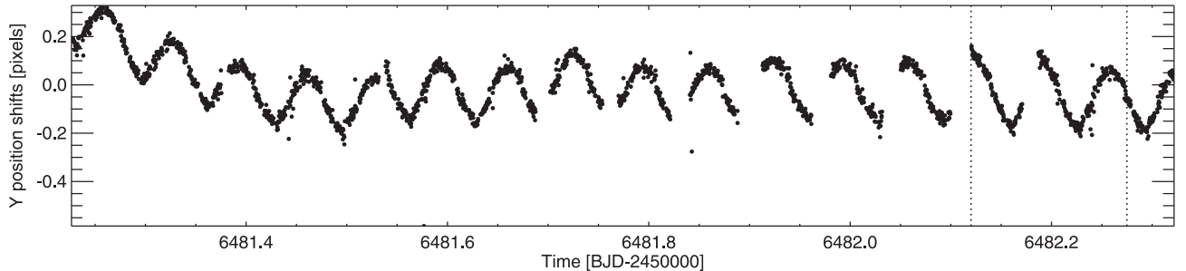
Figure 4. Spectral shifts in Y . Displacement of the spectrum in the cross-dispersion direction. The dotted lines indicate the location and width of the transit pattern described in Section 2.1.2.
