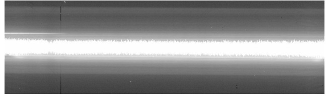
Figure 1. 2D raw extracted spectrum. This spectrum is a sample from our programme PID13180. The degree of saturation and scattered light from the star are both clearly visible.
