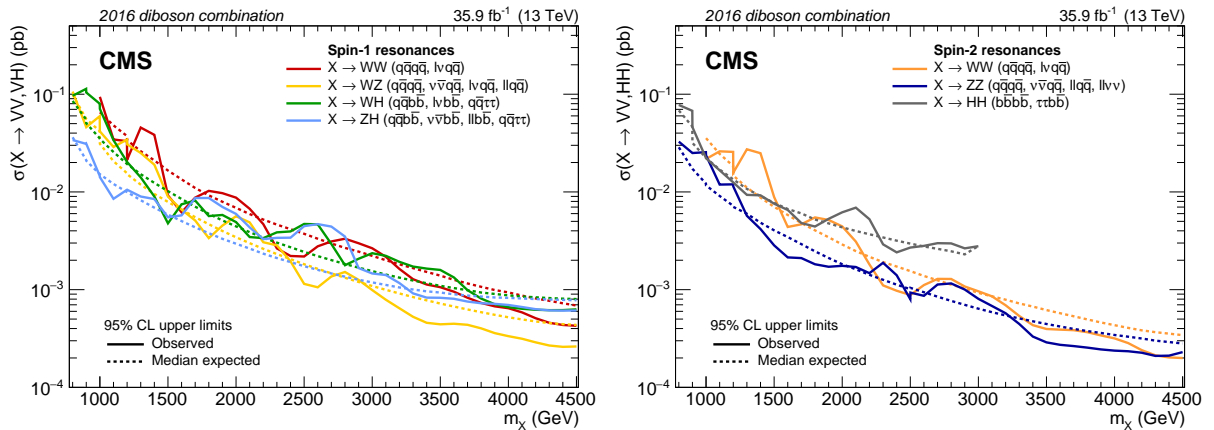
Figure 1: Observed and expected 95% CL upper limits on the product of the cross section and branching fraction of a spin-1 (left) or spin-2 resonance (right) decaying to a pair of SM bosons.
