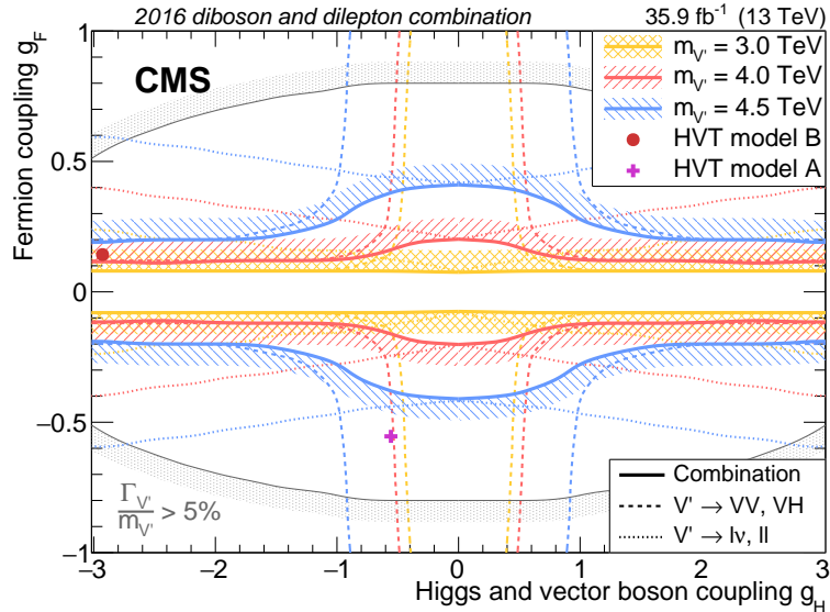
Figure 4: Observed exclusion limits on the couplings of heavy vector resonances to fermions and SM vector bosons and the Higgs boson for the statistical combination (solid lines) of the dilepton (dotted lines) and diboson channels (dashed lines). Three resonance masses hypotheses (3.0, 4.0, and 4.5 TeV) are considered. The hatched bands indicate the regions excluded. The areas bounded by the thin gray contour lines correspond to regions where the resonance widths ( \Gamma_{V'} ) are predicted to be larger than the average experimental resolution (5%).
