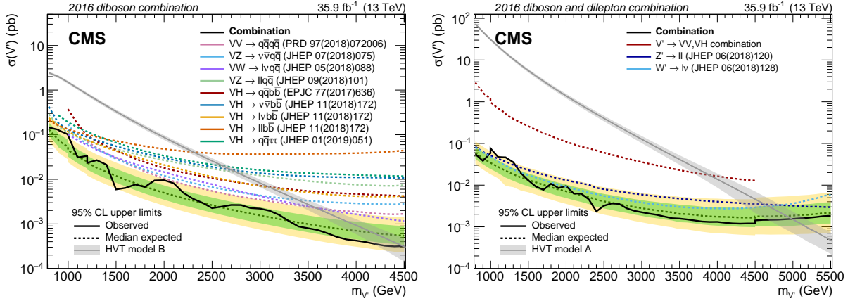
Figure 3: Observed and expected 95% CL upper limits on cross sections as a function of the HVT triplet mass for the combination of all channels in the HVT model B (left) and model A (right). The inner green and outer yellow bands represent the \pm 1 and \pm 2 standard deviation variations on the expected limit. The solid curves surrounded by the shaded areas show the cross sections predicted by HVT models A and B and their uncertainties.
