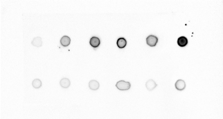
Alpha-synuclein filament dot blot
