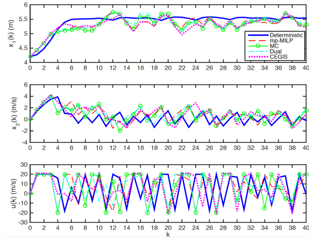
Fig. 1. Eventually maintaining the position between 5-6m in 3 s, using different approaches to solve the optimization problem (3). The blue line shows performance when zero disturbance is assumed.
