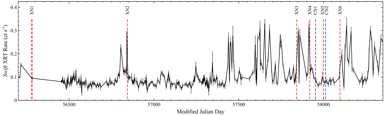
Figure 1. The long-term lightcurve X-ray lightcurve seen by Swift XRT since October 2012. The timing of the NuSTAR observations, which define the broad epochs considered here, are indicated by the red dashed lines for coordination with XMM-Newton , and blue dashed lines for coordination with Chandra . The period after MJD \sim 57400 shows enhanced variability, which is covered by a number of our broadband observations.
