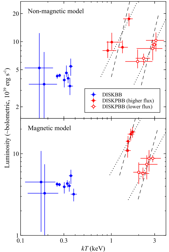
Figure 6. 0.001–100 keV ( i.e. \sim bolometric) luminosity vs temperature for both the DISKBB (blue) and DISKPBB (red) components from our multi-epoch spectral analysis with the models assuming the accretor is non-magnetic (top) and magnetic (bottom). No clear relation is seen for the DISKBB component (although this may be related to modeling issues, see Section 4). However, in both cases the results for the DISKPBB component appear to show distinct tracks at high and low luminosities (observed fluxes above and below F_{0.3-40.0}^{\text{obs}} = 5 \times 10^{-12} \text{ erg cm}^{-2} \text{ s}^{-1} ; full and open symbols, respectively), both of which are broadly consistent with L \propto T^4 (indicated with the dashed lines), and also with L \propto T^2 (dotted lines).
