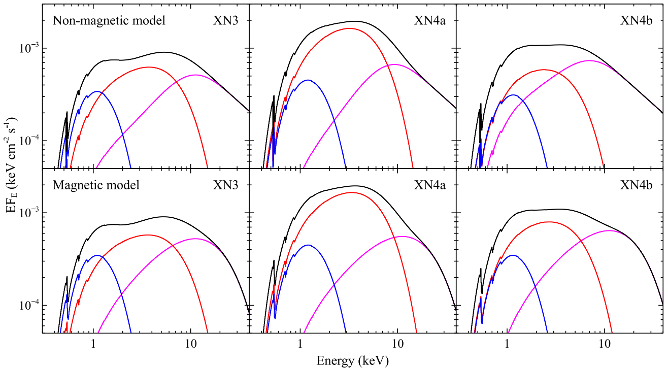
Figure 5. Examples model fits for the non-magnetic accretor ( top panels ) and the magnetic accretor ( bottom panels ) models. We show the fits for epochs XN3 (representing the low-flux end of the broadband spectra; left panels ), XN4a (the high-flux end of the broadband spectra, middle panels ), and XN4b (one of the intermediate flux spectra; right panels ). For both models, the total model is shown in black, the cooler DISKBB and the hotter DISKBB components are shown in blue and red, respectively (in the black hole case, the DISKBB component is shown as it would appear prior to the application of the SIMPL convolution model), and the highest energy component (either SIMPL or CUTOFFPL) is shown in magenta. For the black hole model, the contribution from SIMPL has been calculated by subtracting the unmodified DISKPB component from the combined SIMPL \otimes DISKPB contribution to the fit.
