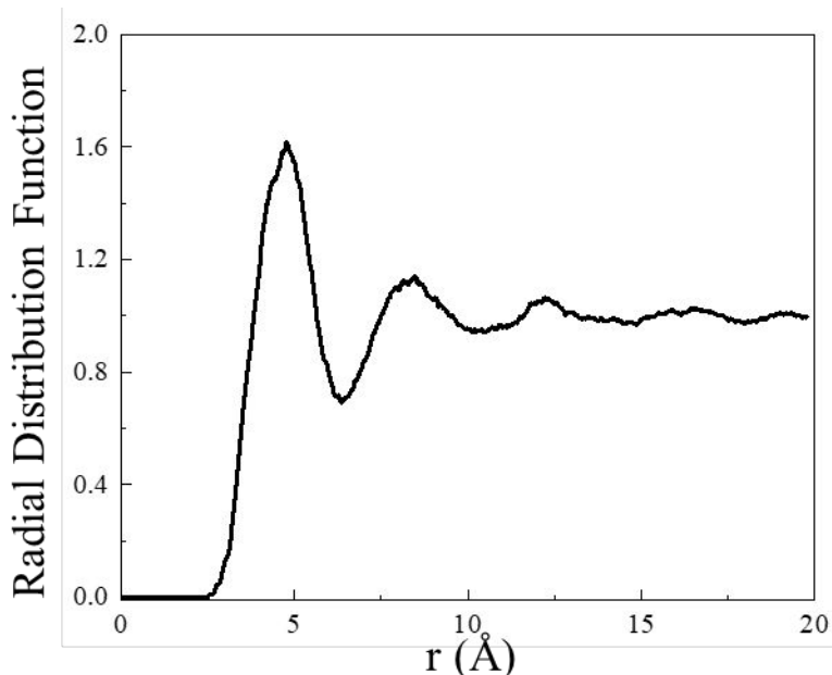
Figure S1. The computed radial distribution function of the NM-NCNO 2 mixture system at 273 K using center of mass of each molecule.
