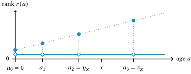
Figure 3.2: Rank Function of FB with Limited Preemption
