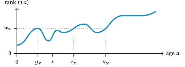
Figure 3.1: Illustration of w_x, y_x, z_x , and u_x
