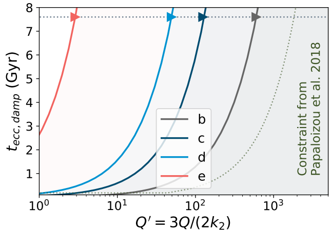
FIG. 5.— The allowable lower limit of Q' for each planet in the TRAPPIST-1 system for the planets for which such constraints can be made, determined by computing the timescale within which the planetary eccentricity will damp to values which cannot be differentiated from zero with current fit precision.
