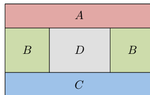
FIG. 1. (color online) Decomposition of the total system into A , B , C , and D . It is possible that a quantum state has no correlation between A and C when looking at only the subsystems A and C but has a strong correlation when looking at them via the subsystem B . This kind of correlation between A and B related to C is measured by conditional mutual information (1). Physically, conditional mutual information characterizes tripartite correlations between A , B and C . A representative example is the topological entanglement entropy [36, 37], which is a special form of the conditional mutual information.
