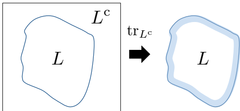
FIG. 3. (color online) Effective Hamiltonian \tilde{H}_L for the reduced density matrix \rho^L . We decompose \tilde{H}_L as \tilde{H}_L = H_L + \Phi_L , where H_L is the original Hamiltonian in L and \Phi_L the effective term that originates outside L . Theorem 3 implies that \Phi_L is exponentially localized around the surface region of L .
