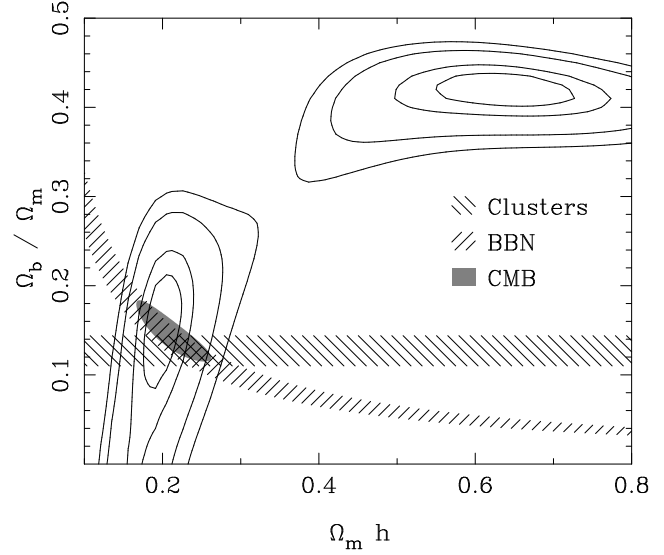
Figure 6. Likelihood surfaces for the best fit linear power spectrum over the region 0.02 h \text{ Mpc}^{-1} < k < 0.15 h \text{ Mpc}^{-1} , as in Fig. 5, but now adding a prior on h : h = 0.7 \pm 10\% . This tightens the constraints. This result is compared to estimates from X-ray cluster analysis (Evrard 1997), big-bang nucleosynthesis (O’Meara et al. 2001) and recent CMB results (Netterfield et al. 2001; Pryke et al. 2001). Note that we have plotted the CMB result following the reasonable approximation that \Omega_b h^2 and \Omega_{\text{cdm}} h^2 were independently determined by each of these analyses.
