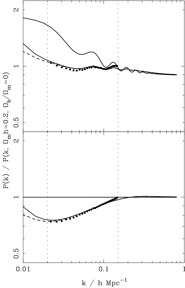
Figure 2. The effect of convolving a linear power spectrum with the 2dFGRS window function. Two model power spectra are compared: The top panel shows a power spectrum including a baryonic component P(k, \Omega_m h = 0.2, \Omega_b / \Omega_m = 0.16) while the bottom panel shows a power spectrum P(k, \Omega_m h = 0.2, \Omega_b / \Omega_m = 0) with no baryonic component. These spectra are divided by a smooth reference model, P(k, \Omega_m h = 0.2, \Omega_b / \Omega_m = 0) . The upper solid lines show the unconvolved power spectra, and the lower solid lines after numerically convolving with the fit to the window function given by Equation 4. The dashed lines show the average power spectrum expected from data which has had the average over-density artificially set to zero (see Section 3.2 for details). Solid symbols show the shape of the average recovered power spectrum from 1000 Gaussian realizations of the density field (with different phases), placed on a 256 \times 256 \times 128 grid at locations covered by the 2dFGRS. Due to the relatively coarse grid used, aliasing swamps the signal at k > 0.15 h \text{ Mpc}^{-1} , and data are only shown for the range of k over which the 2dFGRS power spectrum is fitted (Section 6). This region is delineated by the vertical dotted lines.
