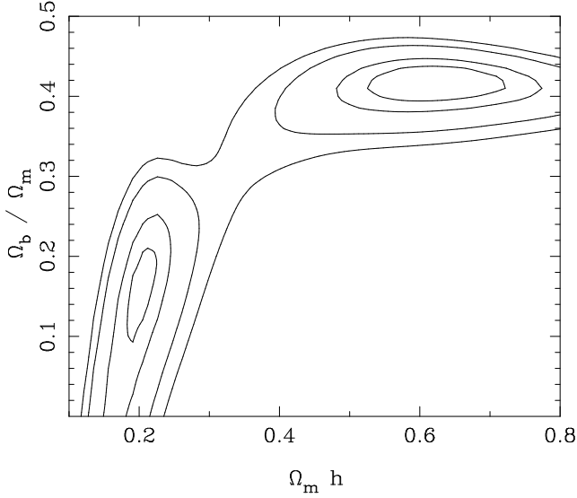
Figure 5. Likelihood surfaces for the best fit linear power spectrum over the region 0.02 h \text{ Mpc}^{-1} < k < 0.15 h \text{ Mpc}^{-1} . The normalization is a free parameter to account for the unknown large-scale biasing. Contours are plotted at the usual positions for one-parameter confidence of 68%, and two-parameter confidence of 68%, 95% and 99% (i.e. -2 \ln(\mathcal{L}/\mathcal{L}_{\text{max}}) = 1, 2.3, 6.0, 9.2 ). We have marginalized over the missing free parameters ( h and the power spectrum amplitude) by integrating under the likelihood surface.
