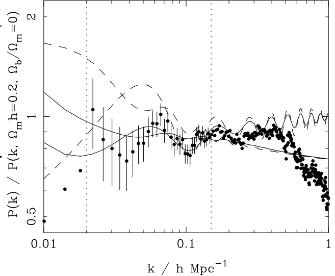
Figure 7. The 2dFGRS data compared with the two preferred models from the Maximum Likelihood fits convolved with the window function (solid lines). Error bars show the diagonal elements of the covariance matrix, for the fitted data that lie between the dotted vertical lines. The unconvolved models are also shown (dashed lines). The \Omega_m h \simeq 0.6 , \Omega_b / \Omega_m = 0.42 , h = 0.7 model has the higher bump at k \simeq 0.05 h \text{ Mpc}^{-1} . The smoother \Omega_m h \simeq 0.20 , \Omega_b / \Omega_m = 0.15 , h = 0.7 model is a good fit to the data because of the overall shape.
