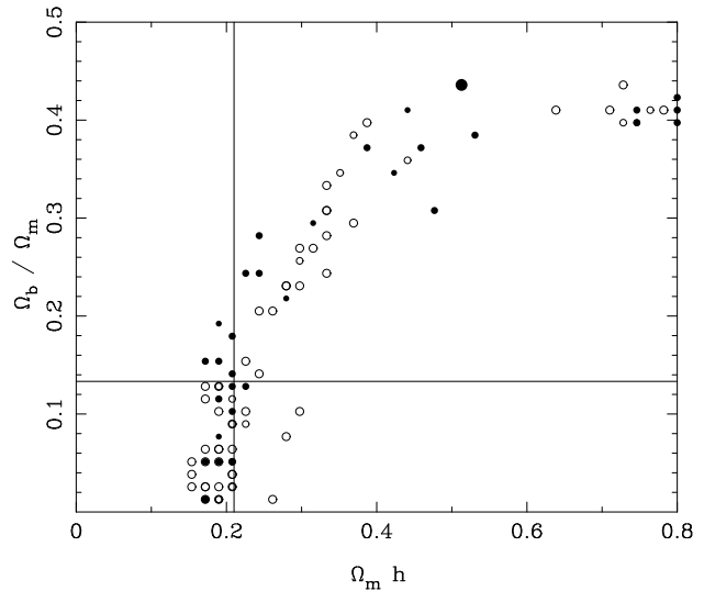
Figure 8. 2D likelihood maxima in the (\Omega_m h, \Omega_b/\Omega_m) plane calculated from 35 redshift-space catalogues drawn from the \Lambda CDM Hubble volume simulation. We have marginalized (by integrating under the likelihood) over h and P(k) amplitude assuming a Gaussian prior h = 0.7 \pm 0.07 and a uniform prior for the amplitude. Primary maxima are given by the solid circles, other maxima with -2\ln(\mathcal{L}/\mathcal{L}_{\text{max}}) < 9.2 (of which there were \sim 1.7 for each catalogue) by the open circles. Primary maxima for which there was no secondary maximum are shown by the large solid circles. The locus of recovered parameters has a similar pattern to that of power spectra with similar shape over 0.02 h \text{ Mpc}^{-1} < k < 0.15 h \text{ Mpc}^{-1} , and is also similar to that seen in the likelihood contours deduced from the 2dFGRS data. Solid lines mark the input parameters for the simulation.
