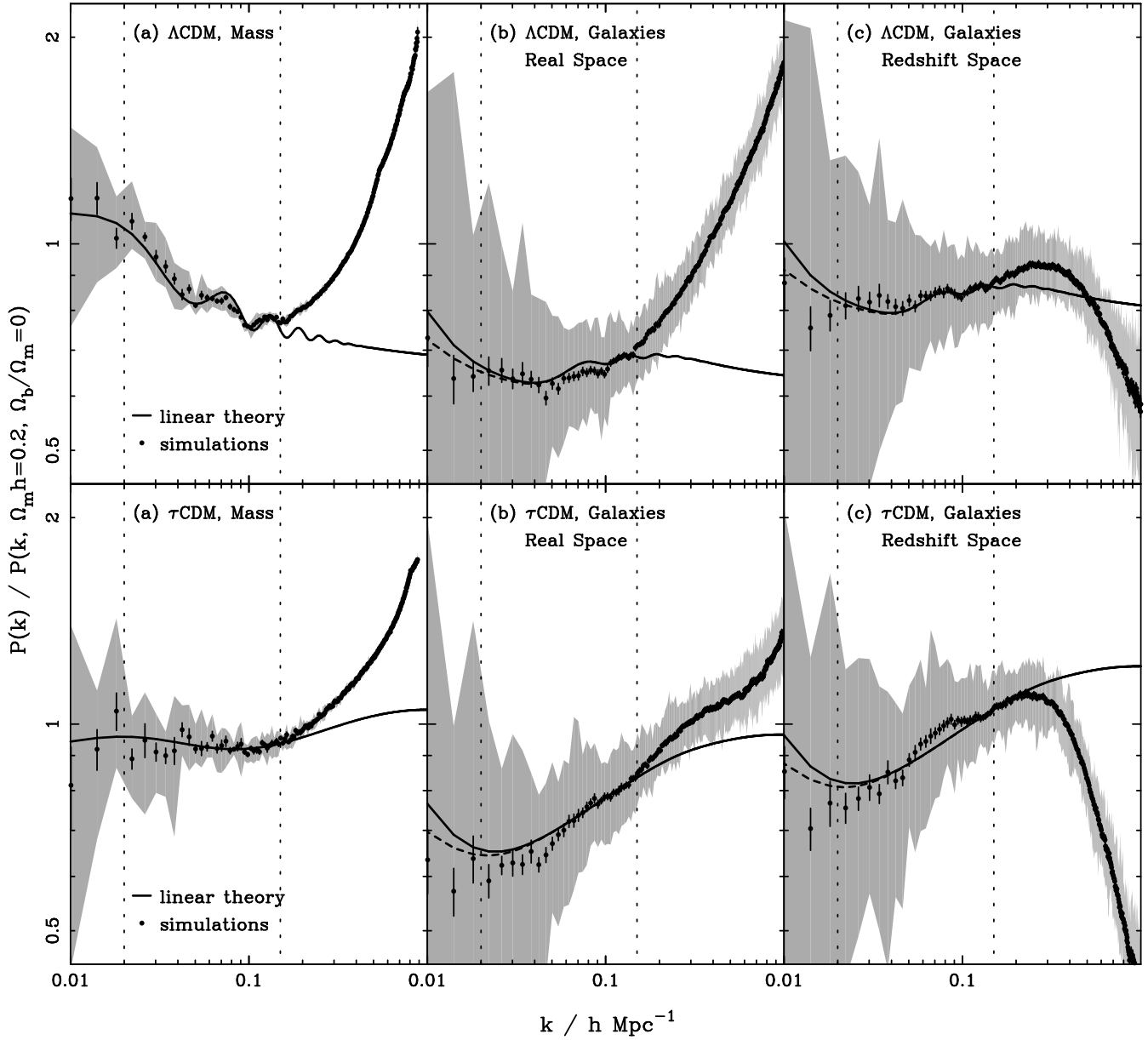
Figure 4. A comparison of power spectra determined from the results of the \Lambda CDM and \tau CDM Hubble volume simulations divided by a P(k, \Omega_m h = 0.2, \Omega_b / \Omega_m = 0) reference model. (a) the average spectrum recovered from the z = 0 distribution of mass in 8 cubes each of side 1500 h^{-1} Mpc ( \Lambda CDM) or 1000 h^{-1} Mpc ( \tau CDM) (solid circles with 1\sigma errors: the extremal data bound the shaded area), compared to the scaled input power spectrum (solid line). Here, the difference between the two is dominated by the non-linear collapse of small-scale structures at k > 0.15 h \text{ Mpc}^{-1} . The \tau CDM mass power spectrum is compared to a reference model with \sigma_8 = 0.6 (rather than \sigma_8 = 1.0 ) in order that it has approximately the same normalization as the other data. (b) the average recovered power spectrum from 35 ( \Lambda CDM) and 30 ( \tau CDM) real-space galaxy catalogues sampled from the simulations to match the 2dFGRS window function (solid circles with 1\sigma errors: the extremal data bound the shaded area). These are compared to the linear spectrum convolved with the analytic approximation to the window function given by Equation 4 (solid line). The difference between these two is dominated by both bias (used to create the galaxy catalogue) and non-linear effects. (c) the average recovered power spectra from 35 ( \Lambda CDM) and 30 ( \tau CDM) redshift-space galaxy catalogues designed to fully mimic the 2dFGRS redshift-space sample (solid circles with 1\sigma errors: the extremal data bound the shaded area), and the linear spectra convolved with the window function (solid line). Here, the differences are due to all of the factors listed in Section 3.1. The dashed lines in panels (b) & (c) show the power spectrum expected from data in which the average over-density is artificially set to zero (see Section 3.2 for details). The 0.02 h \text{ Mpc}^{-1} < k < 0.15 h \text{ Mpc}^{-1} region fitted in Section 6.4 is delineated by the vertical dotted lines. In calculating the error in the average power spectra measured from the simulations, we have assumed that the samples are independent. This is not precisely true, and the errors plotted therefore underestimate the true error.
