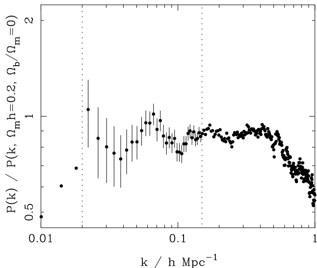
Figure 3. The 2dFGRS estimate of the redshift-space galaxy power spectrum, expressed as the ratio to a linear-theory CDM P(k, \Omega_m h = 0.2, \Omega_b / \Omega_m = 0) power spectrum with n = 1 & \sigma_8 = 1 . These data do not estimate the true power spectrum, but give the power spectrum convolved with the window function (see Section 3.2). Error bars are determined from the diagonal elements of the covariance matrix (calculated in Section 5), for the 0.02 h \text{ Mpc}^{-1} < k < 0.15 h \text{ Mpc}^{-1} data constrained by the vertical dotted lines. This is the region fitted in Section 6.4.
