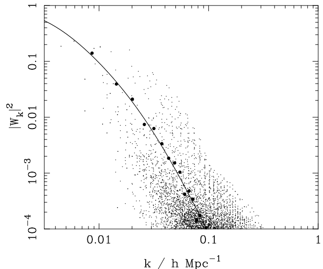
Figure 1. The 2dFGRS window function in Fourier space. The fitting formula of Equation 4 is plotted (solid line) compared to the spherically averaged power obtained by Fourier transforming a random catalogue created to match the 2dFGRS window function (solid circles). This catalogue, containing 5 times as many points as the true galaxy catalogue was placed on a 512 \times 512 \times 256 grid that encompassed all the data. Values from individual grid points are also plotted (dots), and show the anisotropy of the window function.
