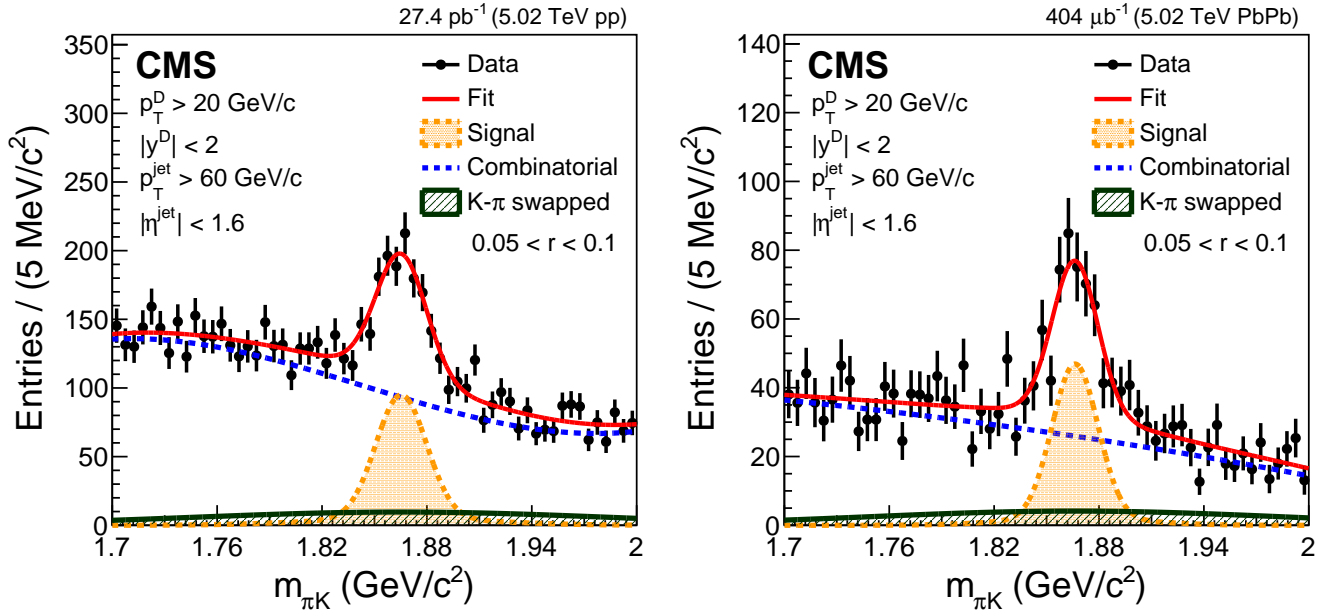
FIG. 1. Examples of raw D^0 candidate invariant mass distributions in pp (left) and PbPb (right) collisions at \sqrt{s_{NN}} = 5.02 \text{ TeV} , for one r interval, 0.05 < r < 0.1 .
