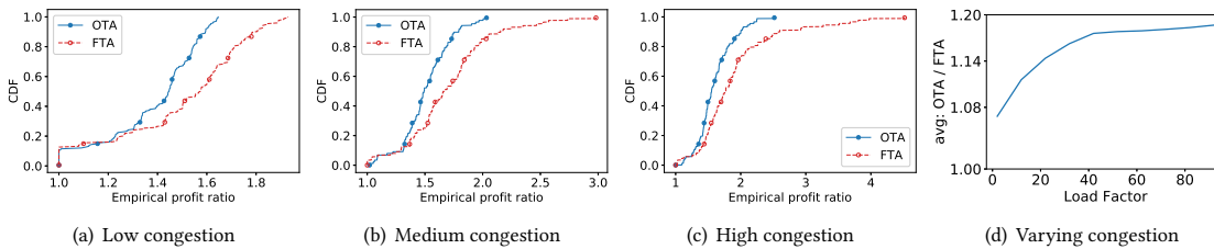
Fig. 2. The CDF of empirical profit ratios of OTA and FTA for (a) low, (b) medium, and (c) high congestion settings. The results show that OTA improves the worst-case profit ratio over FTA by 10.0%, 33.3%, and 44.4% for low, medium, and high congestion settings, respectively. Fig. (d) shows the average % improvement of OTA as compared to FTA as the load factor varies, highlighting a nearly 20% improvement for high load.
