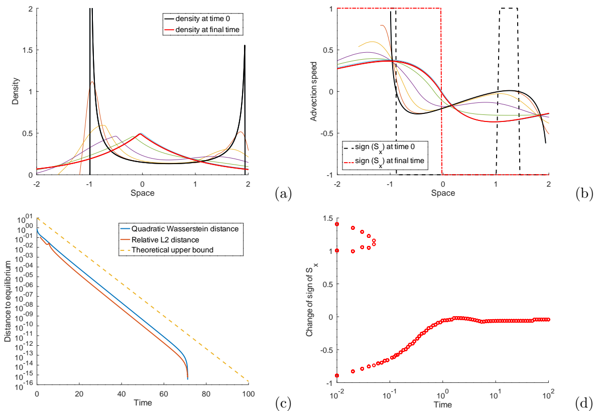
FIGURE 1. Convergence to equilibrium in system (1.1a)-(1.1b): (a) Convergence of the density \rho towards the equilibrium state (1.2). Despite having two peaks initially, it converges towards the stationary profile (1.2). (b) Time evolution of the gradient \partial_x S . The initial configuration S_0(x) has multiple critical points, violating the assumption in Proposition 1.1. However, the convergence still holds, as confirmed by (c), with an actual convergence rate better than the theoretical upper bound \mathcal{O}(e^{-\gamma_0 t}) . (d) Location of the critical points of S (change of sign of \partial_x S ) as a function of time: there are three critical points initially, soon merging into a single \mathbf{x}(t) as assumed in Proposition 1.1. Parameters are: \chi = \alpha = 1 . Discretization parameters are: \Delta\eta = \Delta t = 10^{-2} .
