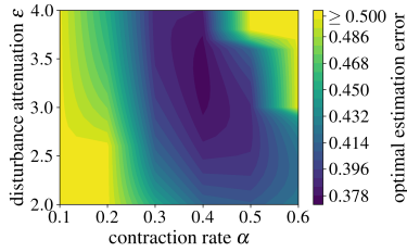
Fig. 3. Optimal steady-state estimation error as a function of \alpha and \epsilon .
