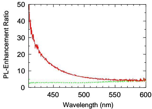
Fig. 3. PL Enhancement ratios demonstrating an increase of enhancement with shorter wavelengths using the silver film. Green dotted line is for gold whereas the red solid line is for silver.
