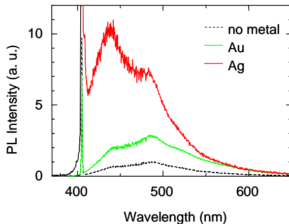
Fig. 2. PL spectra of Coumarin 460 on Ag, Au, and on no metal. Coumarin 460 PL spectra on no metal was normalized to 1.
