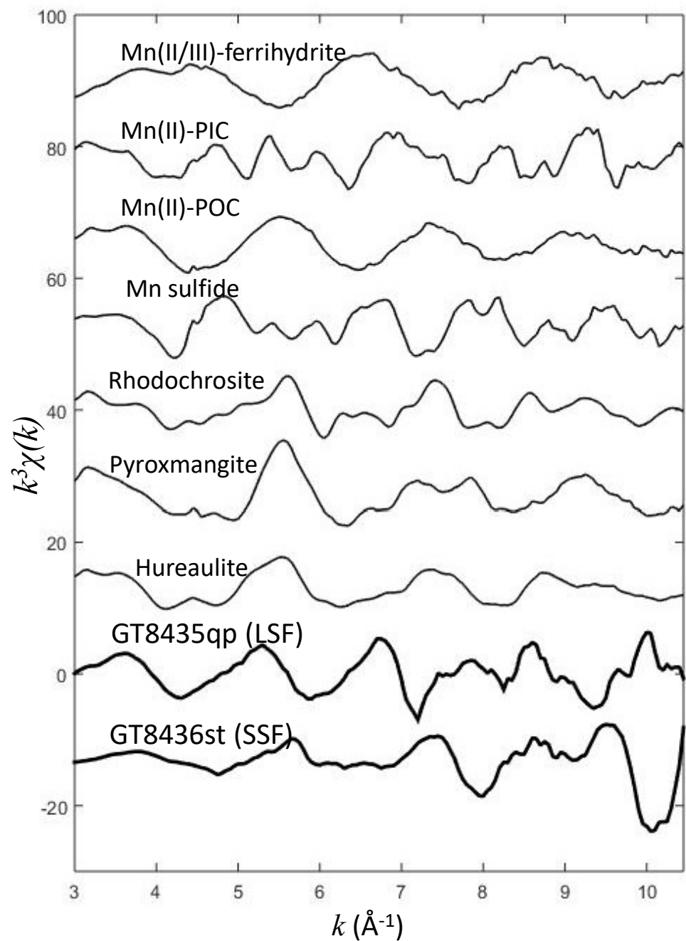
Supplementary Figure 5. Mn EXAFS spectra for Mn-sorbed standards and Mn(II)-bearing minerals (thin black lines) and samples from station 18 with reduced Mn (thick black lines).
