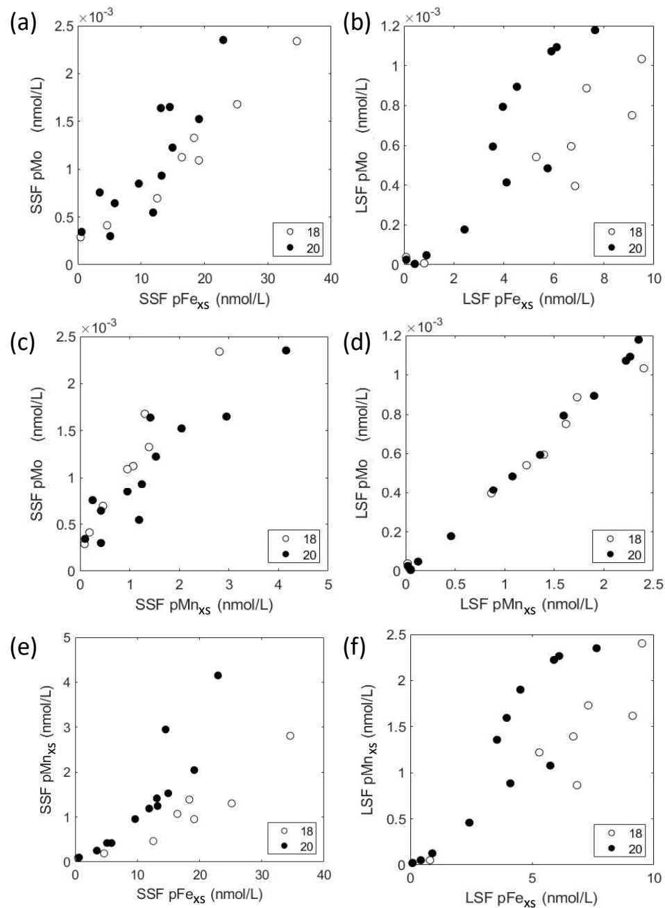
Supplementary Figure 7. Tracer-tracer plots of pMo versus pFe xs , pMo versus pMn xs , and pMn xs versus pFe xs in SSF (a, c, and e) and LSF (b, d, and f) particles in the near-field plume.
