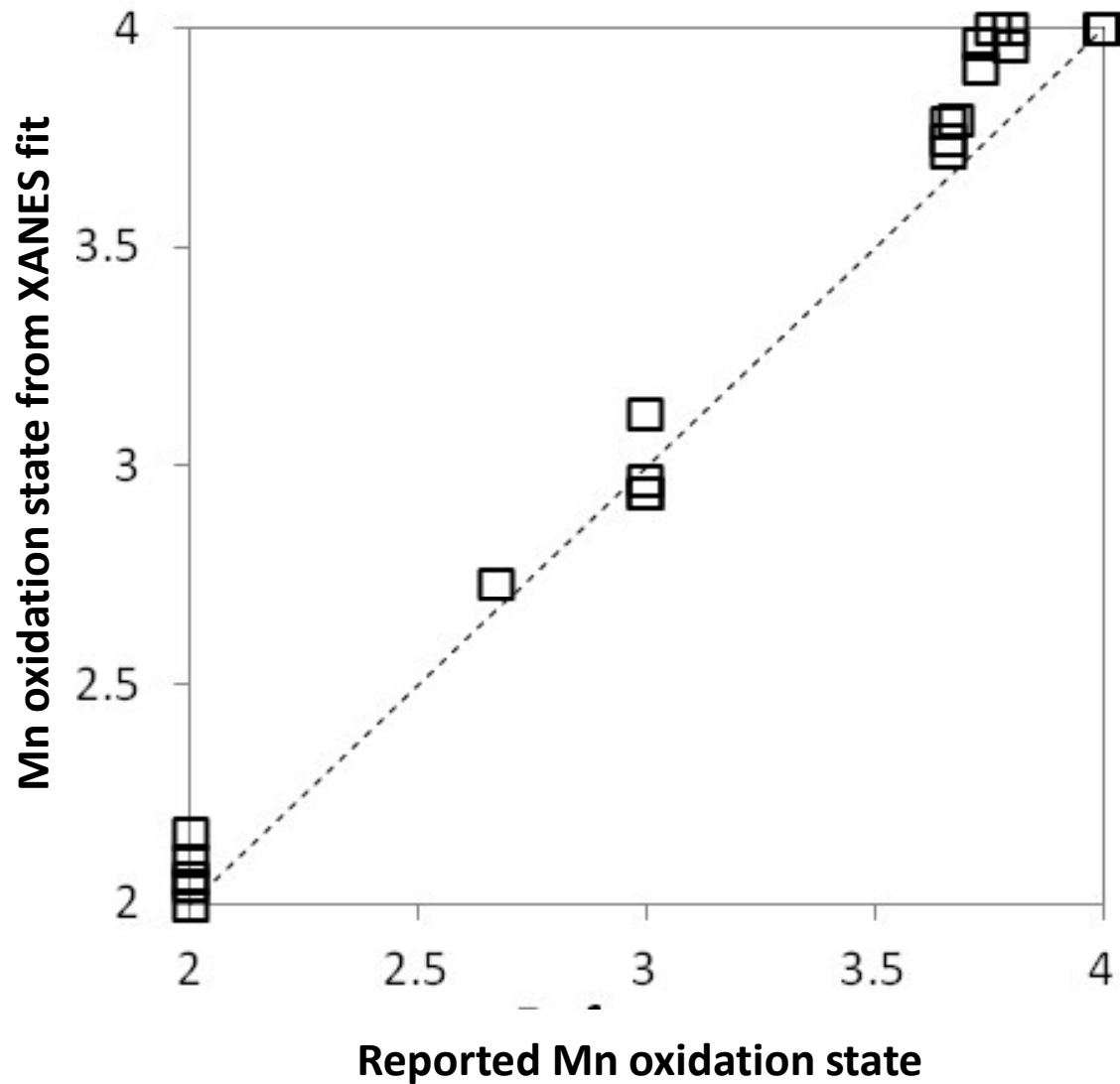
Supplementary Figure 1. Mn oxidation states of reference XANES spectra estimated using linear combination fitting with pyroxmangite, feitknechtite, and \delta -Mn IV O 2 in comparison with the reported values (Manceau et al., 2012; 2014). The dotted line indicates the 1:1 line.
