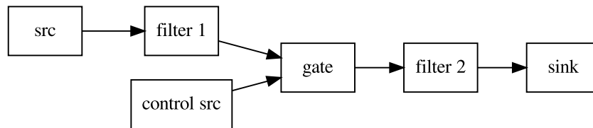
Fig. 2. A basic Gstreamer graph. Data starts at a source, "src", e.g., a file on disk or a network socket, and then is passed through a filter element, "filter 1", which transforms the data, e.g., by performing a low pass filter. A second data stream starts from "control src" and the output of filter 1 is moderated by a gate controlled by the state of "control src". The output of the gate is filtered through "filter 2" and sent to a sink which could be another file on disk or a network socket.
