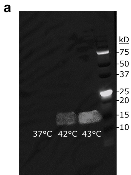
Figure S1 | Western blot to assay for the release of \alpha CTLA-4 upon thermal activation. (a) Unmodified image of the western blot shown in Fig. 3c . The image in Fig. 3c was cropped and inverted to make it fit better into the figure presentation.
