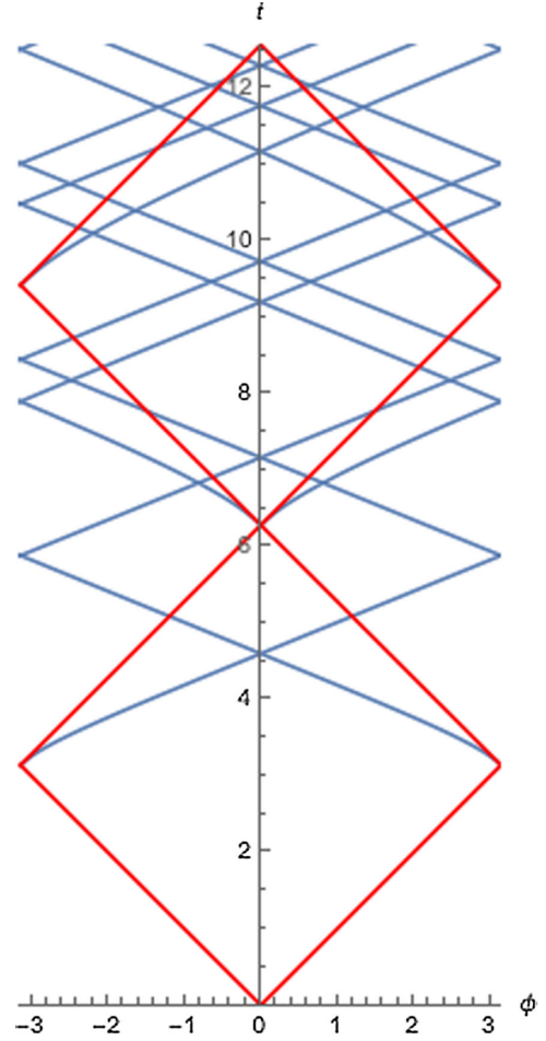
FIG. 2. The intersection pattern of the singularity curves. We see that the number of curves intersecting a given time slice grows linearly with time. Whenever two curves intersect, there is a caustic.
