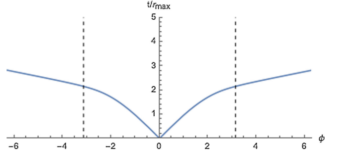
FIG. 3. The light cone in the asymptotically flat case is a single smooth curve. Here we set r_s/r_{\text{max}} = 1/10 .
