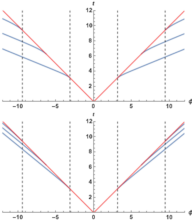
FIG. 1. The locations of the singularities on the boundary. The top figure is for small masses, 4M \sim 0.2 , and the bottom figure is for larger masses, 4M \sim 2 . The angle \phi has period 2\pi , and the dashed lines are identified with each other. The standard light cone is in red, and the new singularities are in blue.
