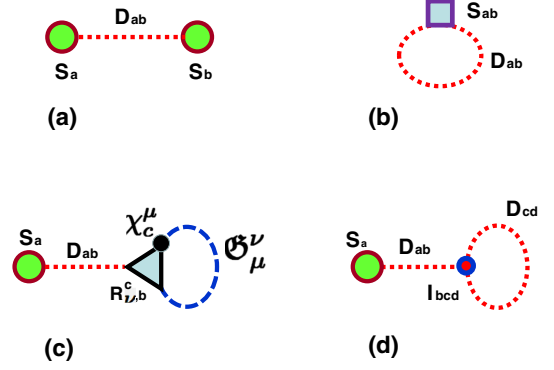
FIG. 4. Diagrams for the matter terms Q_n^{(M)} in the lowest order result for the n th tower in \mathbb{Q} . In (a), the term correlating matter paths, leading to “path bunching,” is shown. The diagrams (b), (c), and (d) show correlations generated between the matter field and the graviton and ghost fields. The solid circles represent derivatives like S_a , the square the second derivative S_{ab} . Dotted lines show the graviton propagator D_{ab} , the dashed line the ghost propagator \mathcal{G}_\mu^\nu ; the small circle represents the graviton 3-point vertex I_{abc} , and the large triangle the 3-point vertex R_{\nu,b}^c . Finally, the solid dot represents the 2-point vertex \chi_c^\mu . For further explanation see text.
