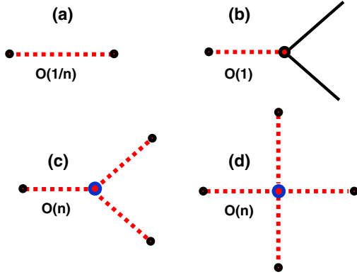
FIG. 3. Diagrams for some of the lower-order vertices in CWL theory, shown along with the order in n that they carry when one sums over n in expressions for the connected generating functional. In (a), we show the basic graviton propagator D^{ab} ; diagrams (b), (c), and (d) show, respectively, a graviton-matter field interaction, a 3-point graviton self-interaction, and a 4-point graviton self-interaction. The smaller solid circle represents the graviton-matter interaction, the slightly larger circle represents graviton self-interactions, the solid line a matter field, and the hatched lines represent gravitons.
