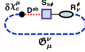
FIG. 6. Diagrammatic representation of the term \delta\chi_c^\mu \mathfrak{G}_\mu^\nu D^{cb} S_{b\phi} R_\nu^\phi in the integrand of Eq. (83). The square shows the derivative \delta^2 S_M / \delta g^b \delta \phi , the dotted line the graviton propagator D_{ab} , and the dashed line the ghost propagator \mathfrak{G}_\mu^\nu . The 2-point vertex R_\nu^\phi is shown as an oval. For further explanation, see text.
