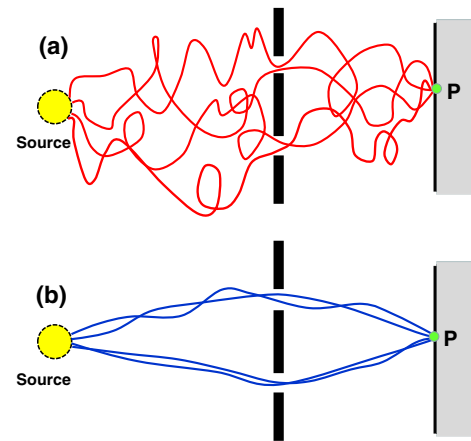
FIG. 1. The effect of interpath CWL gravitational correlations. In (a), some paths are shown for a QM particle moving through a 2-slit system from the source to a point P on the screen. In (b), we have the same arrangement but with CWL correlations between the paths.
