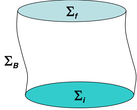
FIG. 2. The boundary hypersurface \Sigma of the spacetime region considered in this paper. It comprises future and past parts \Sigma_f and \Sigma_i , along with a region \Sigma_B at spatial infinity.
