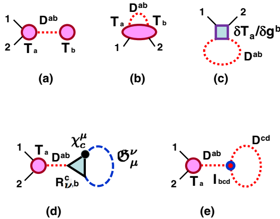
FIG. 5. Diagrams for the different terms in the correlator \langle \phi_1 \phi_2 \rangle^{\text{CWL}} in Eq. (68), between field configurations \phi_1(x) and \phi_2(x) (labeled as ‘‘1’’ and ‘‘2’’ in the diagram, and shown as straight solid line insertions). All terms in Eq. (68) are shown in the order in which they appear, except for the first term \langle \phi_1 \phi_2 \rangle . In (a), we have the ‘‘path-bunching’’ term, while (c) shows the ‘‘seagull’’ contribution, and the diagrams in (d) and (e) show contributions coming from the coupling between the matter field and the graviton and ghost fields. The solid circles represent expectations of stress energies like T_a , the elliptical solid the combined correlator of T_a and T_b , and the square shows the derivative \delta T_a / \delta g^b . Dotted lines show the graviton propagator D_{ab} , the dashed line the ghost propagator \mathfrak{G}_\mu^\nu ; the small circle represents the graviton 3-point vertex I_{abc} , and the large triangle the 3-point vertex R_{\nu,b}^c . Finally, the solid dot represents the 2-point vertex \chi_c^\mu . For further explanation, see text.
