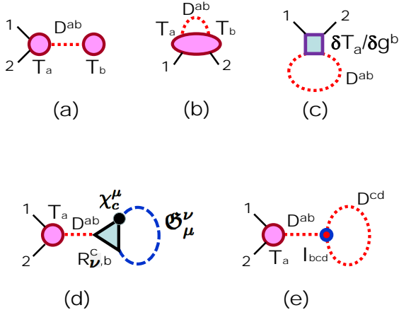
FIG. 5: Diagrams for the different terms in the correlator \langle \phi_1 \phi_2 \rangle^{\text{CWL}} in eqtn. (66), between field configurations \phi_1(x) and \phi_2(x) (labelled as “1” and “2” in the diagram, and shown as straight solid line insertions). All terms in eqtn. (66) are shown in the order in which they appear, except for the first term \langle \phi_1 \phi_2 \rangle . In (a) we have the “path-bunching” term, while (c) shows the ‘seagull’ contribution, and the diagrams in (d) and (e) show contributions coming from the coupling between the matter field and the graviton and ghost fields. The solid circles represent expectations of stress-energies like T_a , the elliptical solid the combined correlator of T_a and T_b , and the square shows the derivative \delta T_a / \delta g^b . Dotted lines show the graviton propagator D_{ab} , the dashed line the ghost propagator \mathcal{G}_{\mu\nu}^c ; the small circle represents the graviton 3-point vertex I_{abc} , and the large triangle the 3-point vertex R_{\nu,b}^c . Finally, the solid dot represents the 2-point vertex \chi_c^\mu . For further explanation see text.
