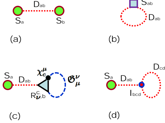
FIG. 4: Diagrams for the matter terms \mathcal{Q}_n^{(M)} in the lowest order result for the n -th tower in \mathbb{Q} . In (a) the term correlating matter paths, leading to “path-bunching”, is shown. The diagrams (b), (c), and (d) show correlations generated between the matter field and the graviton and ghost fields. The solid circles represent derivatives like S_a , the square the second derivative S_{ab} . Dotted lines show the graviton propagator D_{ab} , the dashed line the ghost propagator \mathfrak{G}_\mu^\nu ; the small circle represents the graviton 3-point vertex I_{abc} , and the large triangle the 3-point vertex R_{\nu,b}^c . Finally, the solid dot represents the 2-point vertex \chi_c^\mu . For further explanation see text.
