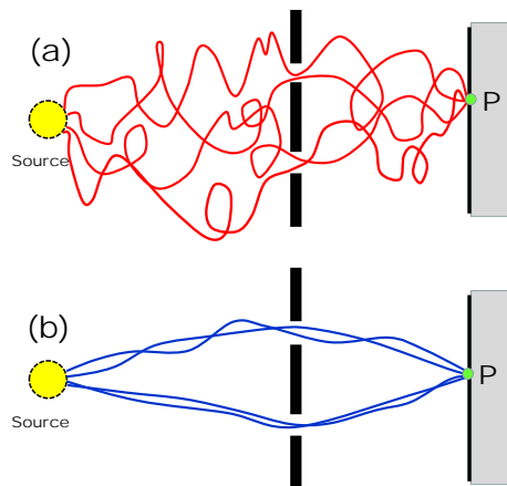
FIG. 1: The effect of interpath CWL gravitational correlations. In (a) some paths are shown for a QM particle moving through a 2-slit system from the source to a point P on the screen. In (b) we have the same arrangement but with CWL correlations between the paths.
