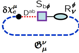
FIG. 6: Diagrammatic representation of the term \delta\chi_c^\mu \mathfrak{G}_\mu^\nu D^{cb} S_{b\phi} R_\nu^\phi in the integrand of eqtn. (81). The square shows the derivative \delta^2 S_M / \delta g^b \delta\phi , the dotted line the graviton propagator D_{ab} , and the dashed line the ghost propagator \mathfrak{G}_\mu^\nu . The 2-point vertex R_\nu^\phi is shown as an oval. For further explanation see text.
