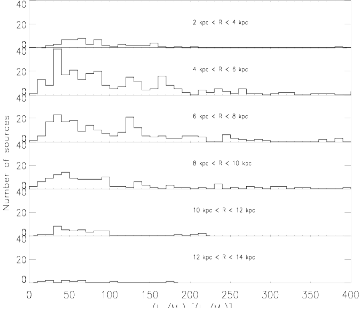
FIG. 8.— IR luminosity to dust mass ratio ( L_{\text{IR}}/M_{\text{IR}} ) as a function of Galactocentric radius, R_G .
