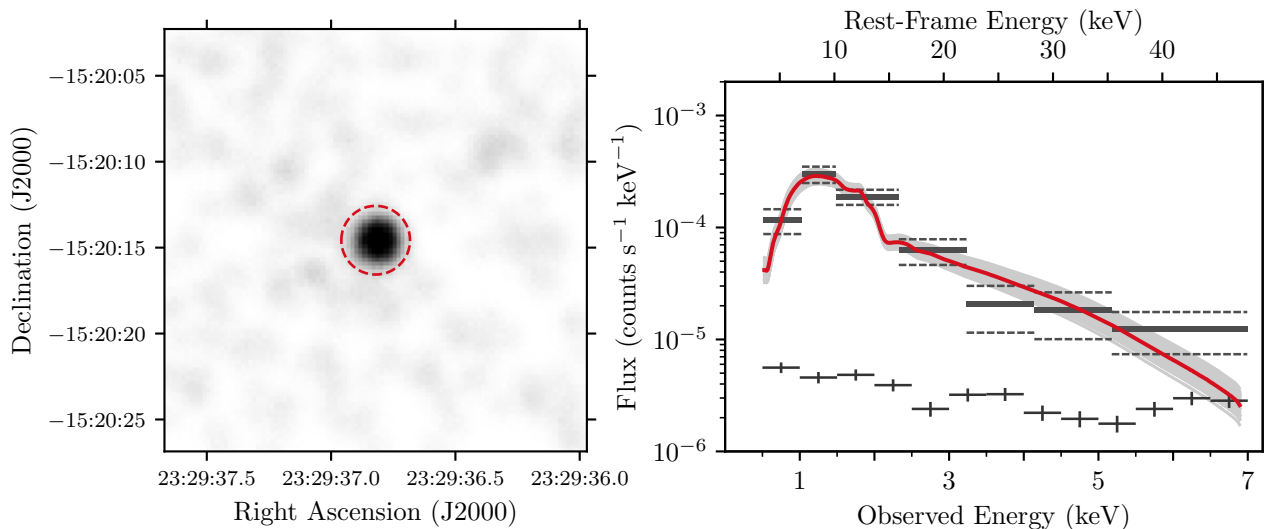
Figure 1. Left: 0.5 – 7.0 keV Chandra observation of PJ352–15, smoothed by a Gaussian kernel of width 0''.75 . The 2''.0 radius extraction region used for photometry and spectroscopy is indicated by the red circle. Right: X-ray spectrum of PJ352–15. Data (dark gray) are binned for ease of display, but were not binned during fitting. The best-fitting spectrum is shown in red, while 100 spectra with \Delta C \leq 2.30 from our Monte Carlo analysis are shown in gray. The background spectrum is shown in dark gray error bars at the bottom.
