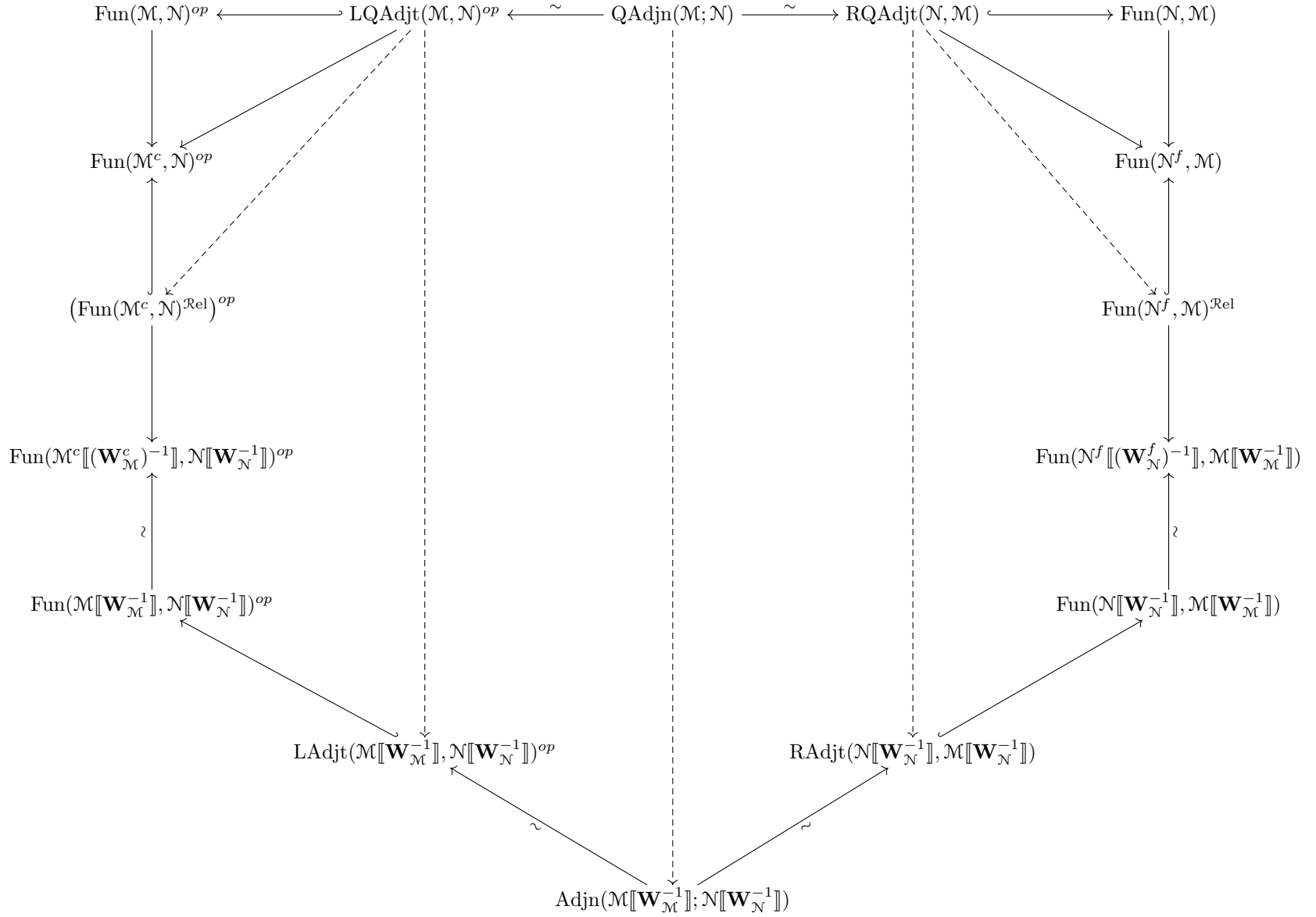
FIGURE 1. The main diagram in the proof of Lemma 4.5.
