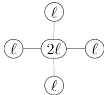
(a) The \widehat{D}_4 Lagrangian quiver when (p_1, p_2, p_3, p_4) = (2, 2, 2, 2) and G = SU(2\ell) .
