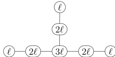
(b) The \widehat{E}_6 Lagrangian quiver when (p_1, p_2, p_3, p_4) = (1, 3, 3, 3) and G = SU(3\ell) .
