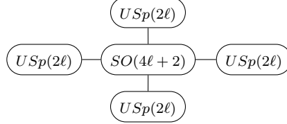
(a) The Lagrangian quiver description of \widehat{D}_4(SO(4\ell + 2)) .
