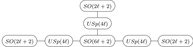
(b) The Lagrangian quiver description of \widehat{E}_6(SO(6\ell + 2)) .
