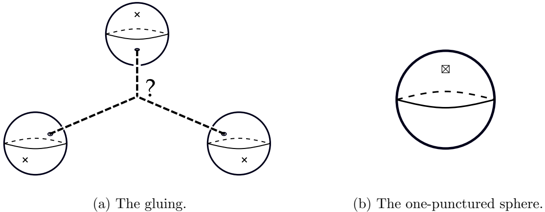
Figure 2.2: The trivalent gauging of the common G flavor symmetry of \mathcal{D}_{p_1}(G) , \mathcal{D}_{p_2}(G) , and \mathcal{D}_{p_3}(G) is depicted in (a). Each of the three theories has an interpretation as a sphere with a irregular puncture and a regular puncture, where the latter contributes the flavor symmetry, G . The regular punctures are glued together to gauge G , and the three irregular punctures, denoted by crosses, remain. In known examples, this is equivalent to a one-punctured sphere, depicted in (b), where the puncture (denoted as a boxed cross) is formed by coalescing the three irregular punctures.
