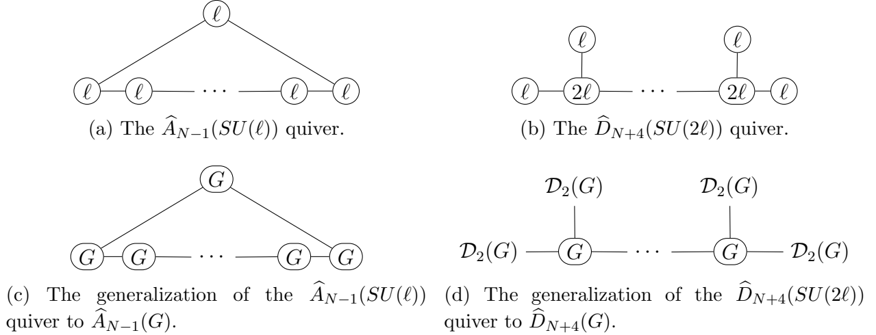
Figure 5.1: We show the affine quivers associated to the affine Dynkin diagrams \widehat{A}_{N-1} and \widehat{D}_{N+4} , together with the generalizations that we consider. We can take N \geq 1 and N \geq 0 respectively, and we remind the reader that an integer K inside a gauge node implies the gauge group SU(K) .
