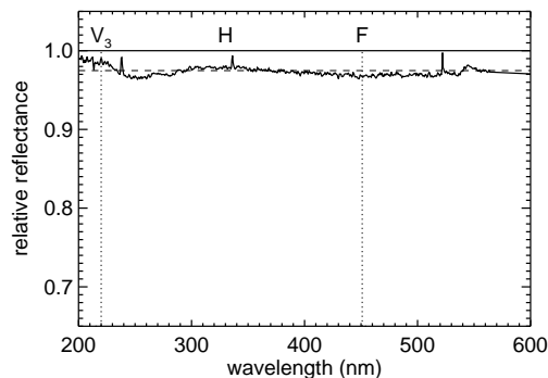
Figure 4. A spectrum of pure indium foil irradiated for three hours at identical conditions to the NaCl experiments divided by the spectrum of unirradiated indium (equivalent to the turquoise-colored curves in Figure 1). Irradiation of indium causes no features larger than \pm 1.5\% to appear in the reflectance spectrum.
