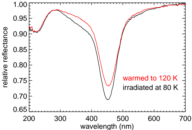
Figure 2. NaCl irradiated at 80 K for 5 hours (black) compared to the same sample after termination of radiation, raising of the temperature to 120 K, and photobleaching at Europa-like fluxes for 2 hours. The F-center absorption decays and shifts redward with higher temperatures and photobleaching, the H-center absorption appears to dissipate entirely, and the V_3 absorption remains unchanged.
