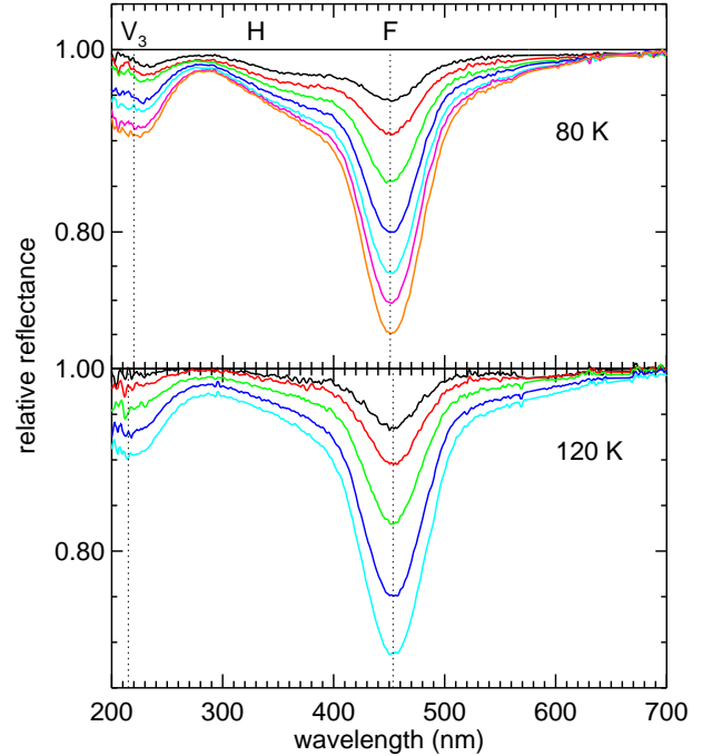
Figure 1. The spectrum of NaCl irradiated at 80 and 120 K with 10 keV electrons. Spectra are shown relative to the spectrum of unirradiated NaCl, which is expected to be nearly spectrally flat through this region. The irradiation times are 15 minutes (black), 30 minutes (red), 1 hour (green), 2 hours (blue), 3 hours (tourquoise), 4 hours (magenta), and 5 hours (orange). For the 80 K irradiation, dashed lines at 220 and 451 nm show the central wavelengths of the color centers, while at 120 K these shift to 453 and 215 nm.
