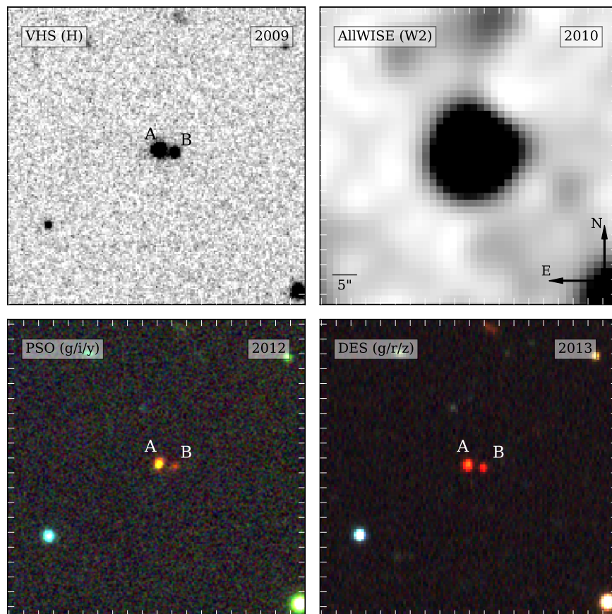
Figure 1. Survey images of CWISE J0146–0508AB. From top left to bottom right; VHS ( H ), AllWISE ( W2 ), Pan-STARRS1 3-color ( g/i/y ), and DES 3-color ( g/r/z ). While it is difficult to resolve CWISE J0146–0508AB in the AllWISE image, it is clearly resolved as a double in the VHS, Pan-STARRS, and DES images. Note also that the reddish colors of each component in the Pan-STARRS1 and DES images indicates very red optical colors, typical of cold brown dwarfs. Each image is 1' \times 1' .
