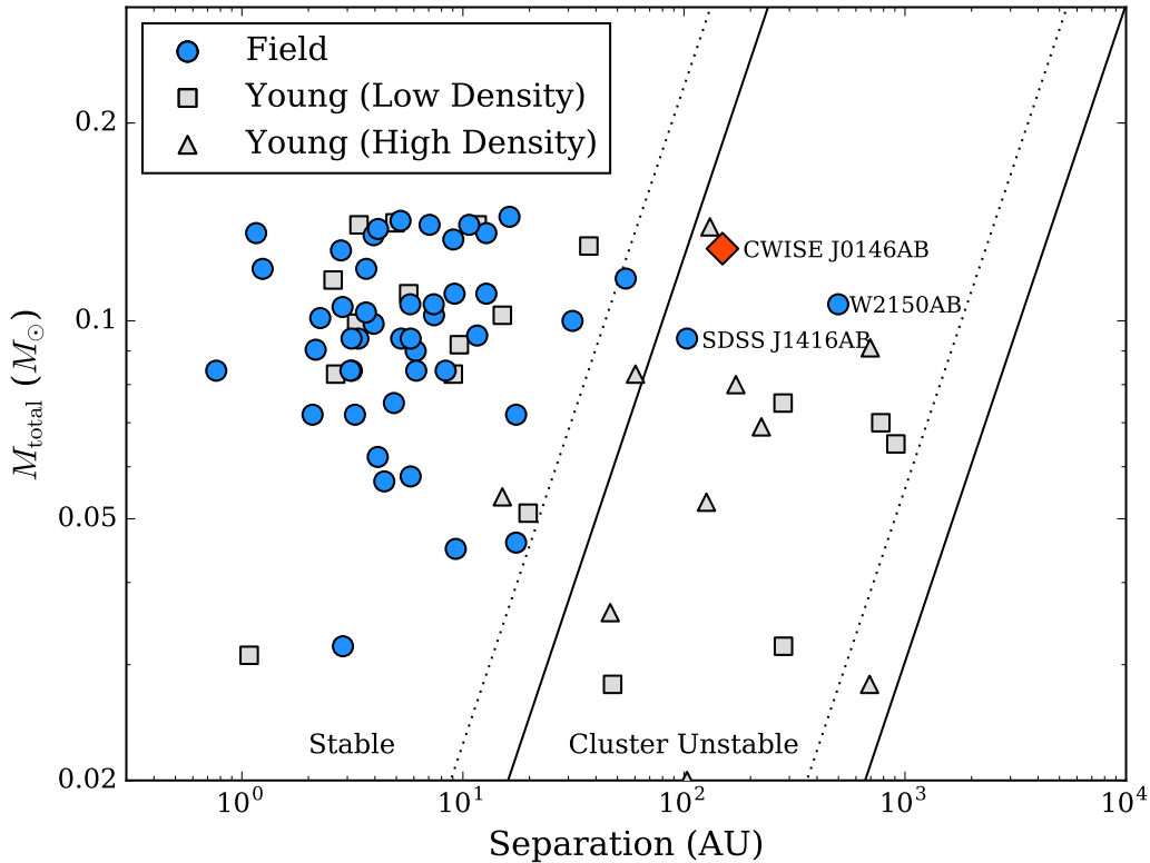
Figure 3. Separation versus total mass for all resolved binaries from Faherty et al. (2020), Strampelli et al. (2020) and De Furio et al. (2021) where each component has a mass less than <0.075 M_{\odot} . Field age pairs are represented by blue circles, while young binaries from dense regions (e.g., ONC) are shown as gray triangles and young binaries from low-density regions (e.g., Taurus, Chamaeleon, \rho Ophiucus) are shown as gray squares. Dotted and solid lines show the instability regions defined in Close et al. (2007), with dotted lines representing the maximum bound separations for cluster (left) and field (right) due to diffusion and solid lines representing maximum separations due to close, catastrophic encounters. These regions are most relevant to the young objects in high-density star-forming regions.
