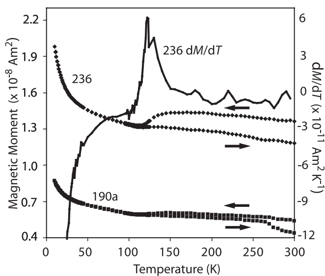
Fig. 1. Low-temperature cycling of two subsamples [236 (upper curves, ♦) and 190a (lower curves, ■)] from ALH84001 after exposure to a saturating field at 300 K. Shown is the moment of the samples in a quenched (<0.2 mT) field as they progressively cooled from 300 K to 10 K and then warmed back up to 300 K. Also shown is the computed first derivative of the moment of 236 with respect to temperature dM/dT (solid line). The peak value of dM/dT specifies the Verwey transition at 122 K for 236 and 119 K for 190a (latter derivative data not shown).
