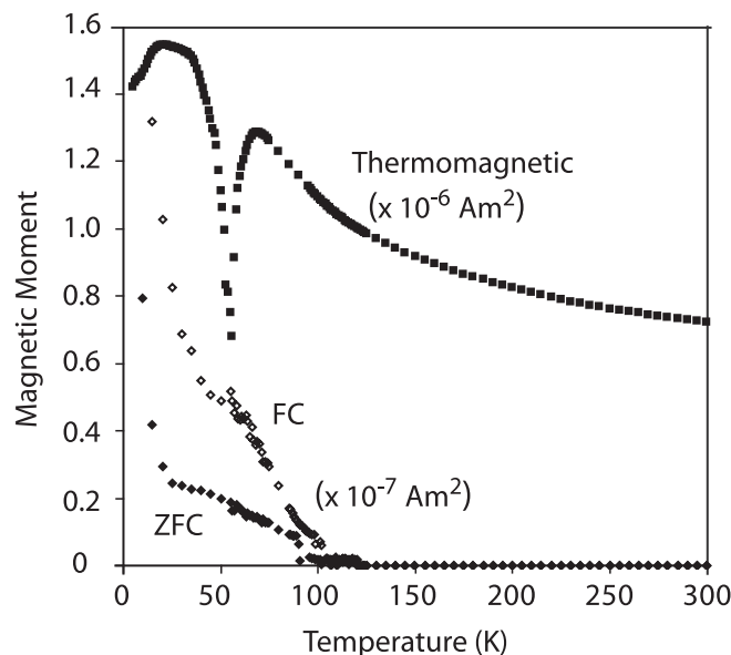
Fig. 3. Low-temperature data on ALH84001 chromite: Moskowitz test data and moment while immersed in a 5-T field. The upper and lower curves are after FC and ZFC treatments, respectively (see Fig. 2). The chromite's \approx 90 K Curie point and an unusual magnetic transition at \approx 55 K are marked (both reproducible in multiple measurement runs).
