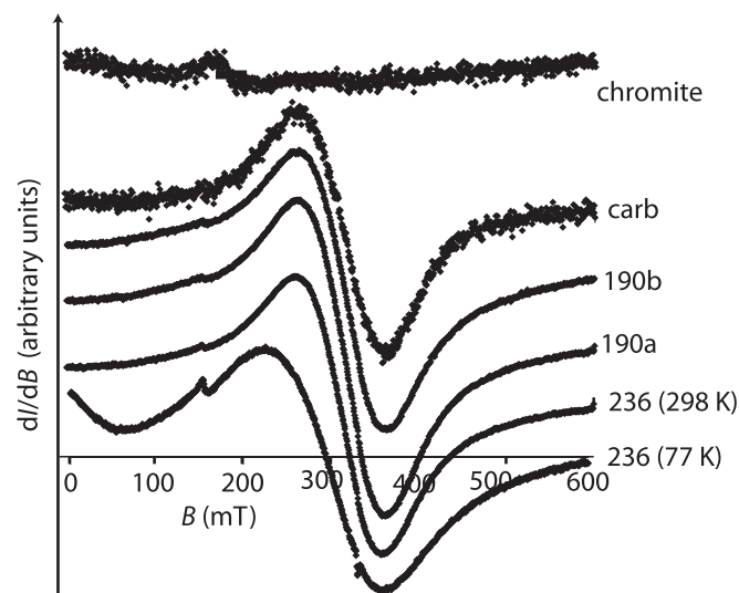
Fig. 4. Selected FMR spectra on ALH84001. Shown is the derivative of the microwave (9.3 GHz) absorption I with respect to the intensity of the applied dc field B (in arbitrary units), plotted as a function of the intensity of the field, B (in mT). The amplitude of each spectrum has been arbitrarily scaled to fit the plot. All data were taken at 298 K except for the lowermost 77 K spectrum.
