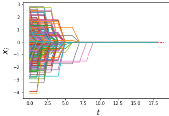
Figure 1. A typical simulation of our hypergraph BCM on the complete hypergraph with N = 500 nodes. Each curve traces the evolution of one node's opinion. We draw the initial opinions from the normal distribution \mathcal{N}(0, \sigma^2) with \sigma = 1.2 . We set the confidence bound to c = 1 . We have reduced the number of time steps by requiring that the hyperedge that we choose at time 0 is concordant. The opinion state converges to consensus.
