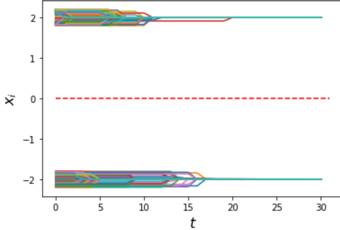
Fig. 3: A typical simulation when the conditions of Theorem 3.18 are satisfied. There are N = 1000 nodes, which we assign to two equal-sized communities. We generate the hypergraph on which we run our BCM from a (p, q, M) -HSBM with p = 1 , q = 1 , and M = 2 . The confidence bound is c = 1 . The initial opinions of the nodes in community 1 are x_i(0) \sim \mathcal{U}(1.8, 2.2) , and the initial opinions of the nodes in community 2 are x_i(0) \sim \mathcal{U}(-2.2, -1.8) . In the limit state, all nodes in community 1 have opinion \gamma_1 \approx 2 and all nodes in community 2 have opinion \gamma_2 \approx -2 . This polarized opinion state is an absorbing state.
