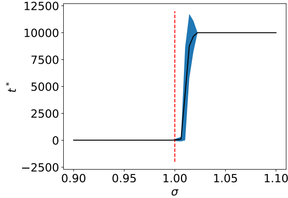
Fig. 6: Empirical convergence time of our BCM on the complete hypergraph with 50,000 nodes and opinions that we seed independently using x_i(0) \sim \mathcal{N}(0, \sigma^2) . We consider all uniformly-spaced values \sigma \in [0.9, 1.1] with a step size of \Delta\sigma = 0.004 . The empirical convergence time t^* is the first time that the discordance function of the opinion state satisfies d(V, \mathbf{x}) < 10^{-5} . If the system does not reach such an opinion state by t = 10^4 , we record t^* as 10^4 . We simulate 20 trials for each value of \sigma . The black curve gives the mean of t^* over the trials, and the blue area depicts one standard deviation from the mean. We include a dashed red line at \sigma^2 = 1 = c for reference.
