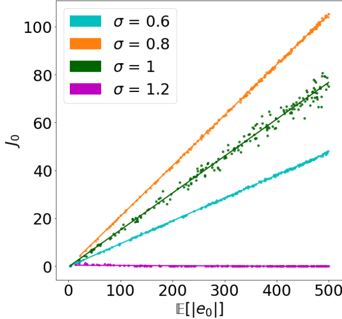
Fig. 7: Empirical evidence for the linear relationship between \mathbb{E}[J_0] and \mathbb{E}[|e_0|] , where J_0 is the number of opinion jumps that occur at time 0 and the hyperedge e_0 is the hyperedge that we choose uniformly at random at time 0. In this numerical experiment, the initial opinions are normally distributed with a mean of 0 and standard deviation of \sigma , which takes values of 0.6, 0.8, 1, and 1.2. For each \sigma , we generate 200 hypergraphs with N = 1000 nodes. To construct the \ell th hypergraph, we choose x_\ell \in [0, 1] uniformly at random and set m_n^{(\ell)} = \binom{N}{i} x_\ell^n . We generate the \ell th hypergraph from the G(N, \mathbf{m}^{(\ell)}) model, which has N nodes and m_n^{(\ell)} hyperedges of size n that we choose uniformly at random. For each hypergraph, we run one step of our hypergraph BCM with confidence bound c = 1 and record the number J_0 of opinion jumps. We run 500 trials for each hypergraph; for each trial, we preserve the hypergraph structure, reset the initial opinions, and run one step of our hypergraph BCM. We record the mean value of J_0 over these 500 trials, and we plot it versus the mean hyperedge size \mathbb{E}[|e_0|] in the hypergraph. Each data point corresponds to the trial results for a single hypergraph for a given value of \sigma . For each \sigma , we plot the line of best fit.
