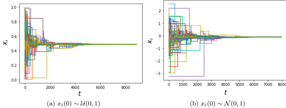
Fig. 5: A typical simulation on the Enron e-mail hypergraph with a confidence bound of c = 1 and nodes with (a) uniformly distributed initial opinions and (b) normally distributed initial opinions. Both of these simulations converge to consensus.
