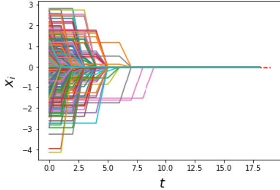
Fig. 1: A typical simulation of our hypergraph BCM on the complete hypergraph with N = 500 nodes. Each curve traces the evolution of one node’s opinion. We draw the initial opinions from \mathcal{N}(0, \sigma^2) with \sigma = 1.2 . We set the confidence bound to c = 1 . We have reduced the number of time steps by requiring that the hyperedge that we choose at time 0 is concordant. The opinion state converges to consensus.
