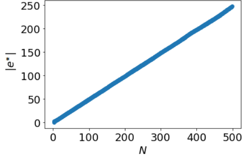
Fig. 2: An estimate of \mathbb{E}[|e^*|] as a function of the number N of nodes, where e^* is the first concordant hyperedge that we select and the initial opinions are normally distributed with a standard deviation of \sigma = 1.2 . The confidence bound is c = 1 . For each possible hyperedge size n \in \{2, \dots, N\} , we run 10,000 trials. For each trial, we randomly draw n opinions from \mathcal{N}(0, \sigma^2) and calculate the sample variance, which equals the discordance of those n opinions. We approximate a_n := \mathbb{P}[d(e, \mathbf{x}(0)) < c \mid |e| = n] by letting \widehat{a}_n be the fraction of trials that result in a concordant set of n opinions. For each N \in \{2, \dots, 500\} , we have that \mathbb{E}[|e^*|] \approx \frac{\sum_{n=2}^N n \widehat{a}_n \binom{N}{n}}{\sum_{n=2}^N \widehat{a}_n \binom{N}{n}} .
