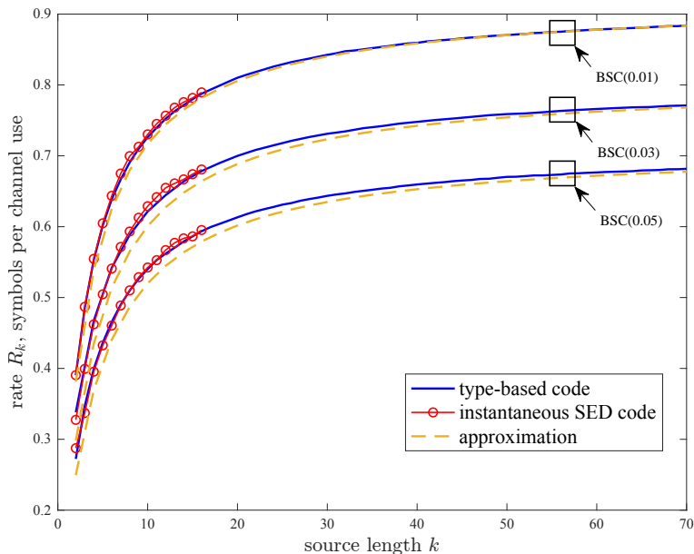
Fig. 9. Rate R_k (symbols per channel use) vs. source length k . The error probability is constrained by \epsilon = 10^{-6} (15). The type-base instantaneous SED code in Section VI-B and the instantaneous SED code in Section V-C operate on k i.i.d. Bernoulli( \frac{1}{2} ) source bits emitted one by one at times t = 1, 2, \dots, k .
