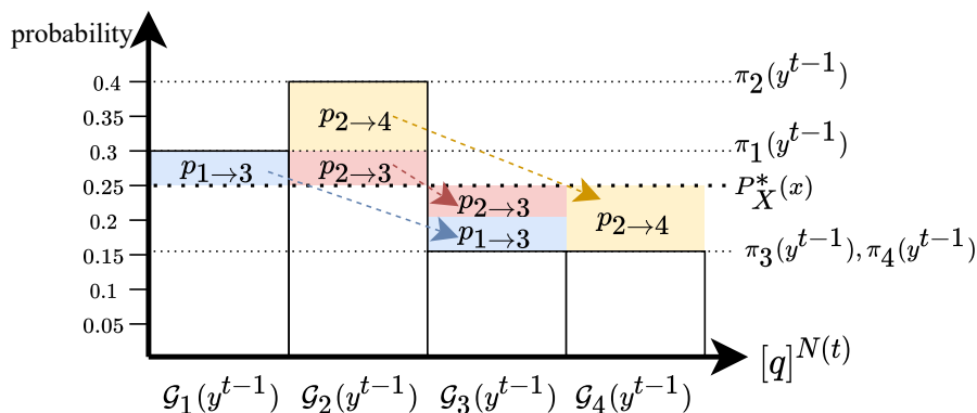
Fig. 4. An example of group partitioning and channel input randomization for a DMC with uniform capacity-achieving distribution P_X^*(x) = 0.25 , \mathcal{X} = [4] . The horizontal axis represents a partition of 4 groups. The vertical axis represents the prior probabilities of the groups. The source alphabet [q]^{N(t)} is partitioned into \{\mathcal{G}_x(y^{t-1})\}_{x \in [4]} such that the partitioning rule (24) is satisfied. Groups \mathcal{G}_x(y^{t-1}) , x \in \{1, 2\} constitute \overline{\mathcal{X}}(y^{t-1}) (26) and groups \mathcal{G}_x(y^{t-1}) , x \in \{3, 4\} constitute \underline{\mathcal{X}}(y^{t-1}) (25). The probabilities \{p_{\bar{x} \rightarrow \underline{x}}\}_{\bar{x} \in \{1, 2\}, \underline{x} \in \{3, 4\}} (27)–(28) used to randomize transmitted group indices are colored. The randomization matches the probability of transmitting group index x \in [4] to P_X^*(x) .
