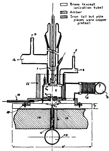
FIG. 1. Side view of the apparatus.
