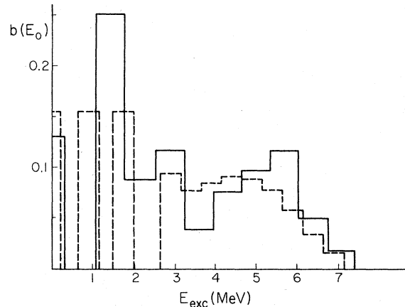
FIG. 3. \beta feeding for the decay of ^{86}\text{Br} , Q = 8.0 MeV. The full histogram shows experimental data of Ref. 15 and the dotted histogram shows the calculated results using Eq. (4).
