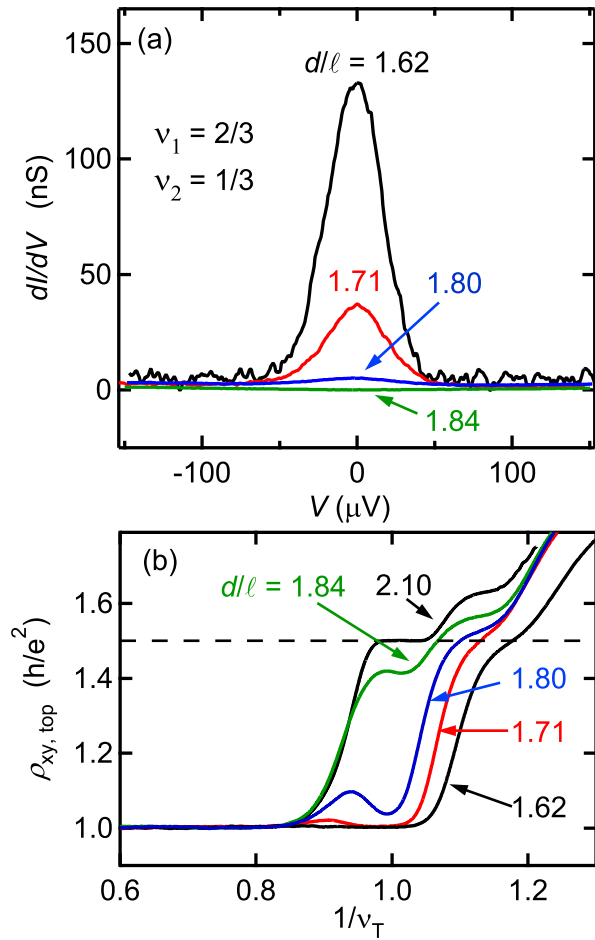
FIG. 7: (color online) Observation of the transition from the interlayer coherent \nu_T = 1 phase to two quasi-independent fractional quantized Hall states. (a) Tunneling conductance spectra at \nu_T = 1 and T = 85 mK at fixed imbalance \Delta\nu = +1/3 (i.e. \nu_1 = 2/3, \nu_2 = 1/3 ). Zero bias peak collapses rapidly as d/\ell increases and interlayer coherence is lost. (b) Hall resistance \rho_{xy, \text{top}} in the top 2DES vs. inverse total filling fraction 1/\nu_T at d/\ell = 1.62, 1.71, 1.80, 1.84 , and 2.10 . For each trace the imbalance at \nu_T = 1 is \Delta\nu = +1/3 . A clear transition from a Hall plateau at h/e^2 to one at 3h/2e^2 is observed at \nu_T = 1 .
