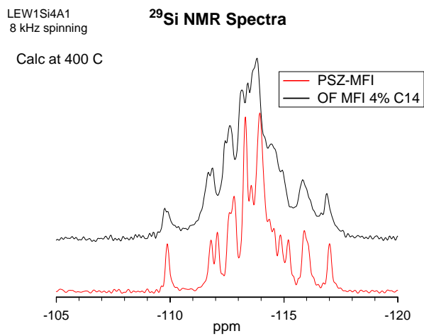
Figure S1. 29 Si MAS NMR spectra of PSZ MFI and OF MFI C14 after calcination at 400 °C.
