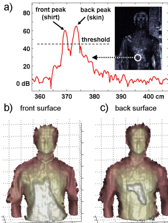
Fig. 5. (a) Power spectrum of individual pixel from dataset of Fig. 4. The pixel location is indicated by a circle in the inset total-power image. Two peaks exceeding threshold come from the subject's shirt and body surface. (b) and (c) Full 3-D reconstructions, after some additional smoothing, of the front and back surface ranges consisting of the identified front and back peaks for each pixel. The concealed handgun is visible as a bulge in the back surface.
