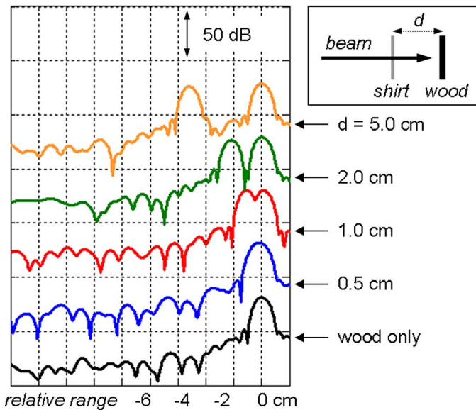
Fig. 3. Range-compressed radar returns (power spectra) of a stretched shirt in front of a flat wooden board at various separations. Two distinct peaks occur once the shirt-wood gap reaches about 1 cm, the practical range resolution of the 600 GHz radar.
