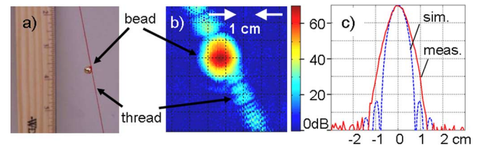
Fig. 2. (a) 3 mm gold-plated bead suspended by a thread. (b) 600 GHz scanned radar image of the bead at 4 m standoff. Even the cotton thread is detected by the radar. (c) Measured horizontal cross-section of the bead's return power through the bead center (solid) and the simulated two-way beam pattern of the main antenna (dashed).
