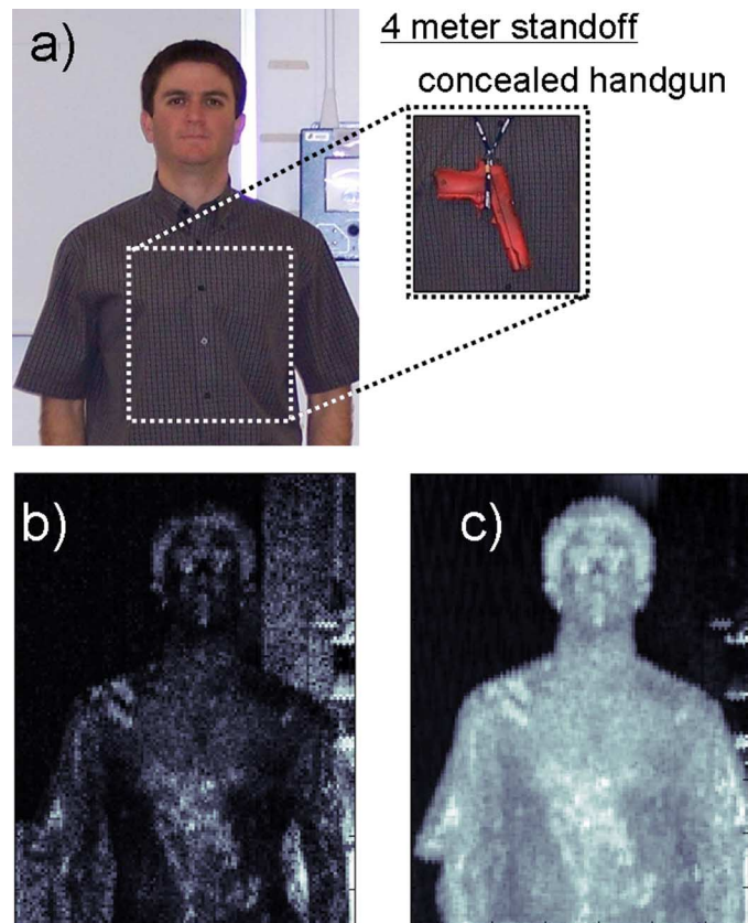
Fig. 4. (a) Target scenario, where a concealed metallic gun replica is hung around the subject's neck and beneath his shirt at 4 m standoff range. (b) Total-power image of the received intensity, on a logarithmic scale, covering the entire final IF bandwidth of 96 kHz (range swath 6.25 m). (c) Image of the received power (log scale) after course filtering over a range swath of 50 cm centered on the subject. Though the image is greatly improved, the concealed gun remains hidden because of shirt and skin clutter signals.
