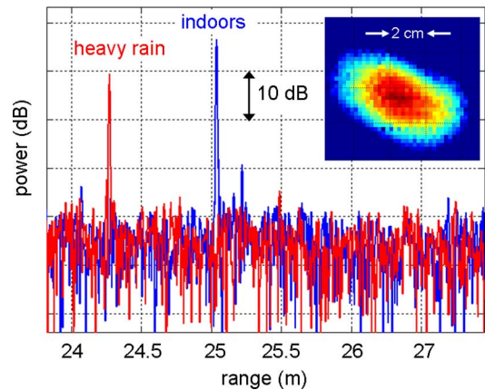
Fig. 7. Comparison of the range-compressed radar returns from a 3 mm gold bead at 25 m standoff, taken in conditions of heavy rain and indoors. Attenuation from rain is only 7 dB. Inset: Beam profile of bead at 25 m standoff. The color scale spans 10 dB of dynamic range, and the beam shape distortion is likely from aberrations in the aperture shape.
