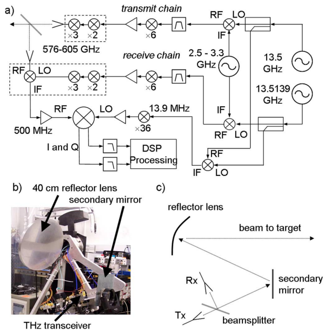
Fig. 1. (a) Block diagram of 600 GHz radar imager. The transmit signal and the receiver LO are generated by multiplying microwave sources by a factor of 36. A 2.5–3.3 GHz chirp, generated by a DDS/PLL synthesizer, results in a final FMCW signal with a 28.8 GHz bandwidth. The submillimeter-wave multipliers and mixer, designed and built at the Jet Propulsion Laboratory, are enclosed by dashed boxes. (b) and (c) Radar photograph and optics schematic.
