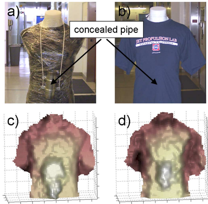
Fig. 6. (a) Target scenario is a plastic mannequin wrapped in damp fabric and plastic at 25 m standoff range. A 2.25 in steel pipe was hung around the neck. (b) During the scan, a T-shirt was placed over the mannequin and pipe. (c) and (d) Front- and back-surface reconstructions revealing the presence of the pipe. The color scale represents range only.
