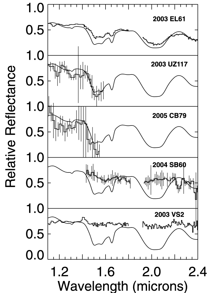
FIG. 2.—Near-infrared spectra of 2003 EL61 and its collisional family members show strong signatures of nearly pure water ice on their surfaces. Shown are the spectra of five KBOs along with a pure crystalline water ice model (Grundy & Schmitt 1998). We observed KBOs 2003 UZ117, 2005 CB79, and 2004 SB60, objects 67, 97 and 221 \text{ m s}^{-1} away from the modeled 2003 EL61 family core (Ragozzine & Brown 2007), to determine if their near-infrared spectra contained the characteristic strong water ice absorptions. Spectra of 2003 UZ117 and 2005 CB79 show strong absorptions at 1.4\text{--}1.6 \mu\text{m} consistent with the presence of high fractions of water ice on their surfaces. In contrast, the spectrum of 2004 SB60 is essentially featureless. The flat spectrum of 2003 VS2 (from Barkume et al. 2008), a typical non-family-member KBO, is shown for comparison.
