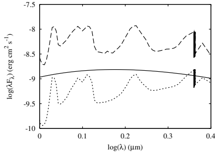
Fig. 3. Comparison of the 2500 K black body emission, added in model II (solid line), with the emission of the inner gaseous disk for two mass accretion rates, 10^{-6} M_{\odot}/\text{yr} (top curve) and 10^{-7} M_{\odot}/\text{yr} (lower curve), over the relevant range of wavelength between 1 and 2.5 \mu\text{m} respectively.
