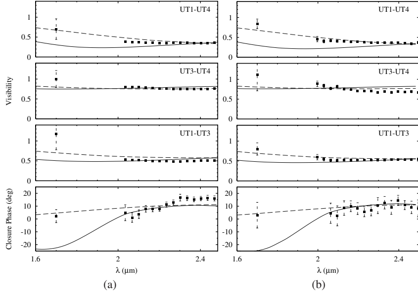
Fig. 1. Spectrally dispersed visibility and closure phase measured across the H ( 1.65 \mu\text{m} ) and K ( 2.2 \mu\text{m} ) bands. Panels a ) and b ) show the data for two different hour angles, \text{HA} = 0.25 \text{ h} and \text{HA} = 0.54 \text{ h} respectively. The three upper panels show calibrated visibilities for the three different baselines as labeled in the figure and described in Sect. 2; corresponding closure phases are plotted in the bottom panel . Visibility errors across K band are between 3 and 5%; H band data has been spectrally averaged to increase signal to noise ratio, the associated error is about 30%. Solid lines correspond to the rim model (I), dashed lines to the gas+rim model (II). Model parameters are reported in Table 1.
