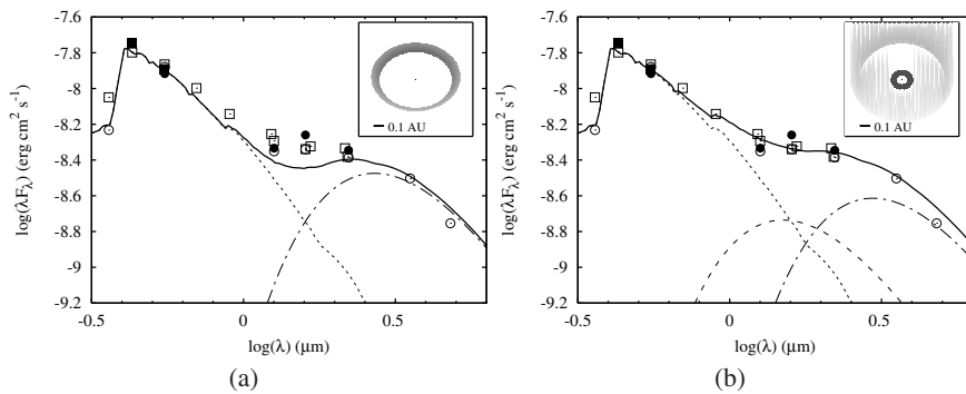
Fig. 2. SED of MWC 758. Symbols show the photometry from the literature corrected for an extinction A_V = 0.4 , R = 3.1 . The stellar spectrum (short-dashed line) is that of a Kurucz model with T_{\text{eff}} = 8000 , \log g = 4 . Panel a ) shows the flux predicted by model I (solid line) composed of the dusty disk rim emission (short-long dashed line) and the star. Panel b ) shows the prediction for model II where an additional black body component is added (dashed line). In each panel the image of the corresponding model is shown in the inset. Refer to Table 1 for model parameters.
