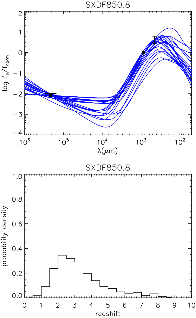
Figure 2. (Top) Spectral energy distribution (SED) of SXDF850.8, where the black squares mark the detections at 850\mu\text{m} and 1.4\text{GHz} used in the photometric redshift calculation. Error bars are 1\sigma , and the arrow at 450\mu\text{m} marks the 3\sigma upper limit derived from our maps. For reference, the SED templates used in the photometric redshift calculation are shifted to z_{\text{phot}}^A = 2.6 and scaled to maximize the likelihood function of detections and upper limit through survival analysis (Isobe, Feigelson & Nelson 1986), and are represented as lines. All the SEDs are compatible within the 3\sigma error-bars of the photometry of the source. (Bottom) Probability distribution for SXDF850.8 derived for the z_{\text{phot}}^A solution, using only the 850\mu\text{m} and 1.4\text{GHz} photometry.
