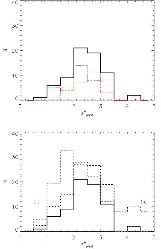
Figure 3. Histogram of modes of the photometric redshift distributions of SHADES galaxies derived from the 1.4\text{GHz}/850\mu\text{m} spectral index. The (black) thick solid-line (shown in the upper and lower-panels) represents the distribution of modes for the 69 galaxies that have been detected at both 850\mu\text{m} and 1.4\text{GHz} . In the upper-panel the (blue) thin dotted-line and (red) thin dashed-line represent the redshift distributions in the LH and SXDF fields respectively. In the lower-panel the black dashed-line (a) and grey dashed-line (b) show the redshift distributions for the full SHADES catalogue, including the 51 sub-mm galaxies undetected at 1.4\text{GHz} . Those SCUBA galaxies with non-detections in the radio are distributed in one of two ways that bracket the range of reasonable options: (a) with equal probability between their calculated lower 90% confidence limits and z = 5 ; and alternatively, (b) between their lower limits and z = 2 , or only at their lower redshift-limits in the cases that these lie at z > 2 .
