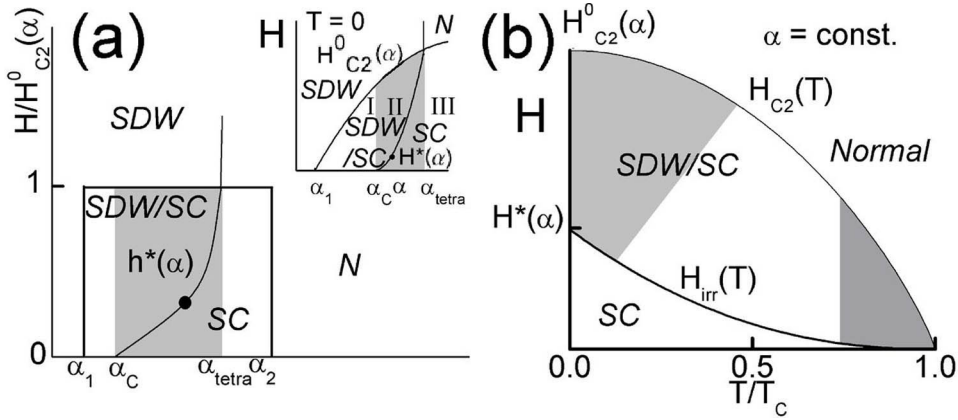
FIG. 1: Schematic phase diagrams of cuprate superconductors with competing SDW and SC: (a) Reduced field h = (H/H_{c2}^0) vs. material parameter ( \alpha ) phase diagram at T = 0 (main panel), transformed from the phase diagram in the inset[10]. Here h^*(\alpha) \equiv H^*(\alpha)/H_{c2}^0 denotes the phase boundary that separates a pure SC from a coexisting SDW/SC phase, and N denotes the normal state. (b) H(\alpha) vs. (T/T_c) phase diagram for a given \alpha value and for magnetic field applied parallel to the ab-planes of the cuprates so that disorder fluctuations can be minimized [32]. The shaded regime between H_{irr}(T \rightarrow 0) and H_{c2}(T \rightarrow 0) is a vortex state associated with strong quantum fluctuations, and that between H_{irr}(T \rightarrow T_c) and H_{c2}(T \rightarrow T_c) is associated with strong thermal fluctuations.
