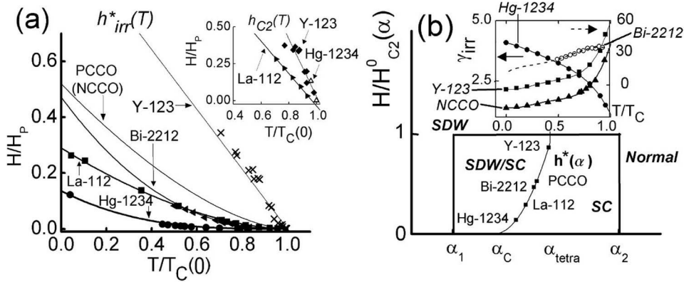
FIG. 3: (a) Comparison of the h^*_{irr}(T) (main panel) and h_{c2}(T) (inset) vs. (T/T_c) phase diagram for Hg-1234, La-112 [32], Bi-2212 [26], NCCO [23, 28], and Y-123 [24, 25] with H \parallel ab -plane, so that the corresponding H_{c2}^0 is limited by the paramagnetic field H_p . (b) Main panel: summary of the proximity of different cuprates to a QCP at \alpha_c . The points along h^* represent the reduced irreversibility fields obtained from data taken on Y-123, PCCO (NCCO), Bi-2212, La-112, and Hg-1234. Inset: Temperature evolution of the anisotropy of the irreversibility fields ( \gamma_{irr} \equiv H_{irr}^{ab}/H_{irr}^c ). The left (right) scale is for solid (open) symbols.
