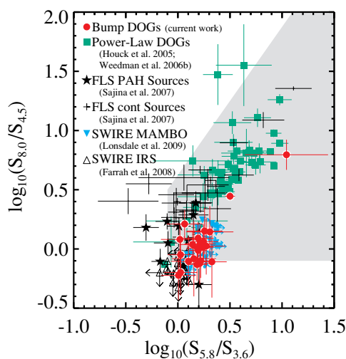
Figure 3. IRAC color-color diagram for z \approx 2 bump DOGs (the red points), the f_{\nu}(24 \mu\text{m}) > 0.75 mJy DOG sample published in Houck et al. (2005) and Weedman et al. (2006; the green points), and the z \approx 2 ULIRG sample from Sajina et al. (2007; the black points). This last sample is divided into PAH-rich sources (the black stars) and PAH-poor sources (error bars only). The wedge used by Lacy et al. (2004) to select AGN-dominated sources is shaded in gray. Bump sources tend to lie in a localized region of IRAC color-color space.
