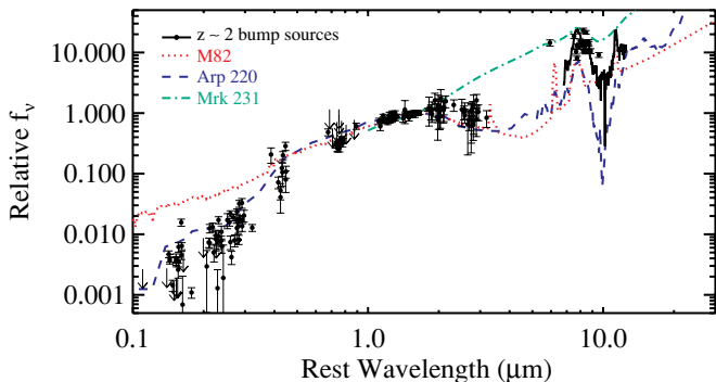
Figure 6. Optical to mid-infrared SEDs of z \approx 2 bump DOGs. Each SED is arbitrarily scaled to have a 1.6 \mu\text{m} flux density of unity. The SEDs of bump DOGs strongly resemble that of Arp 220. As in Figure 1, no color correction has been applied to the Spitzer photometry.
