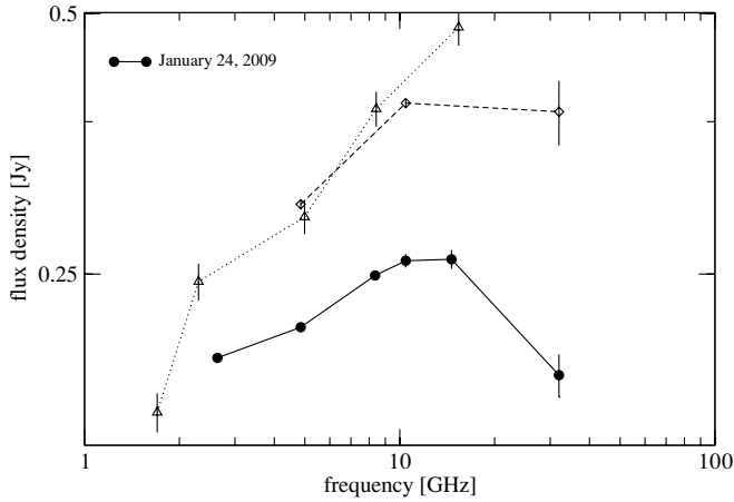
Figure 3. Evolution of the radio spectrum of PMN J0948+0022. Filled circles denote the Effelsberg observations of 2009 January. Archival data are shown in gray: triangles represent VLBA measurements conducted in 2003 October (Doi et al. 2006) and diamonds represent archival Effelsberg measurements obtained in 2006 (Vollmer et al. 2008).
